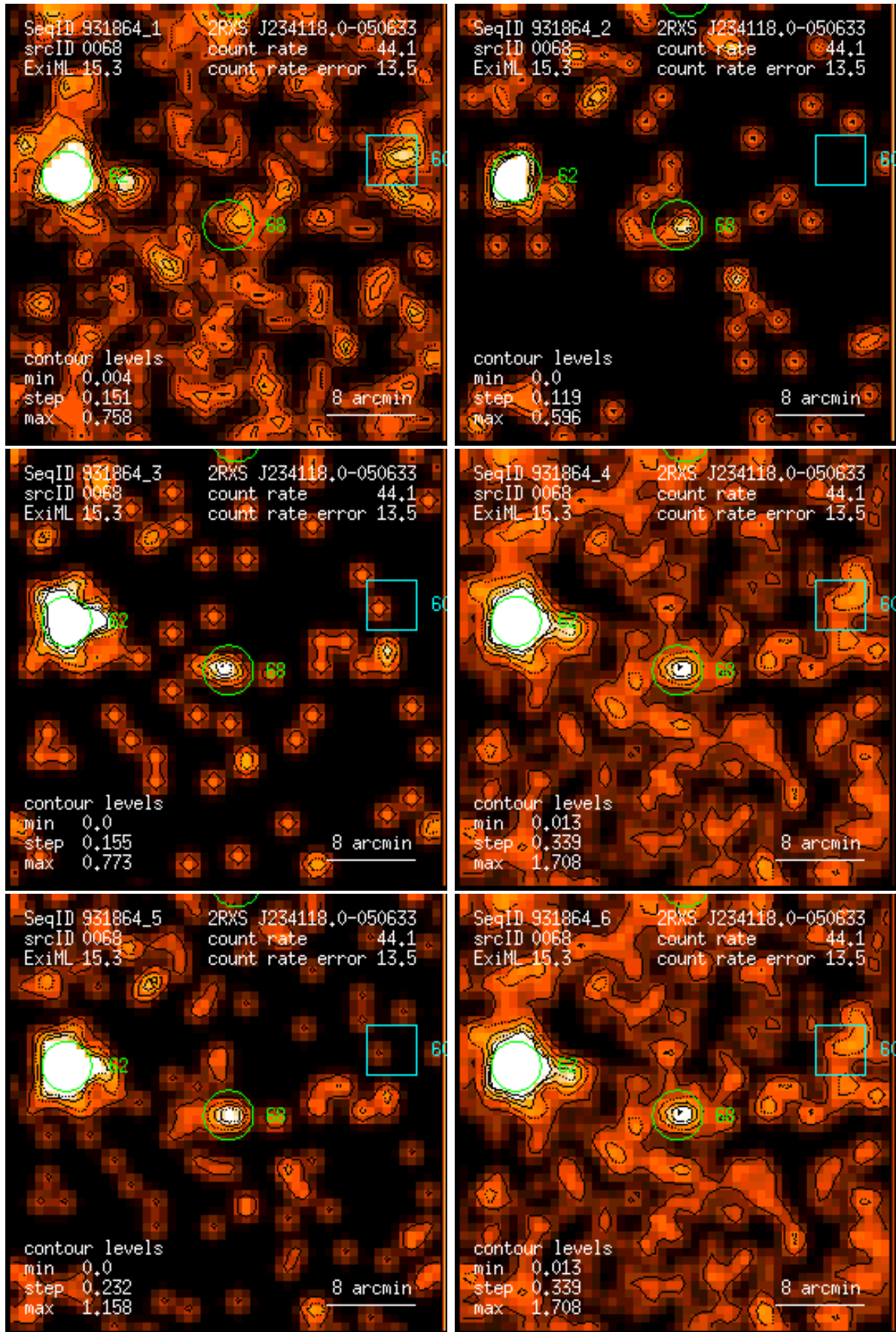
Figure 68: RASS 931864: detection 0068: band rate images, Gaussian filter: (1) PSPC channels 11 – 41, (2) 52 – 90, (3) 91 – 201, (4) 11 – 235, (5) 52 – 201, (6) 11 – 201. Broad band rates in counts/ks. Band rate contour levels in counts/ks/arcmin 2 .
