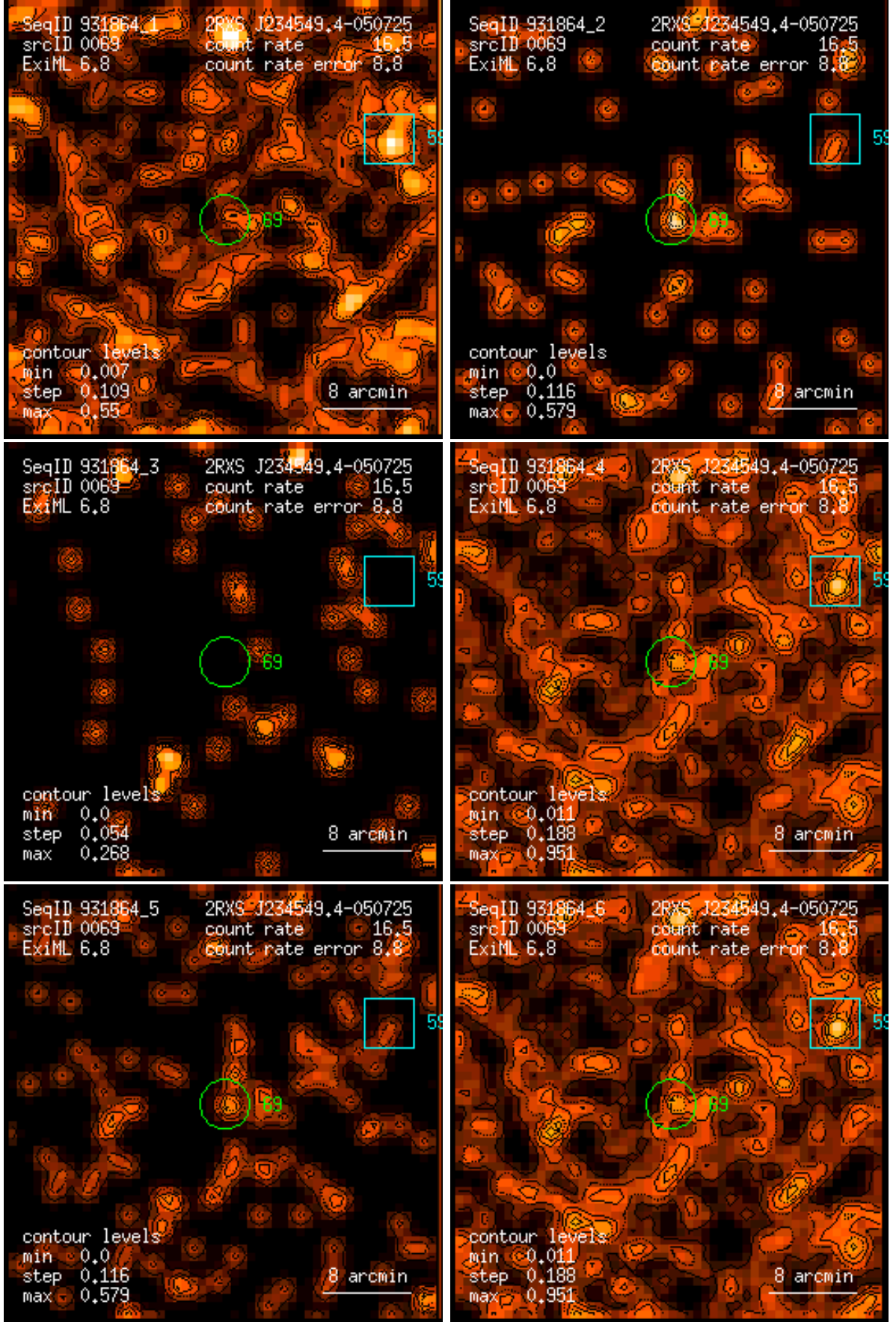
Figure 69: RASS 931864: detection 0069: band rate images, Gaussian filter: (1) PSPC channels 11 – 41, (2) 52 – 90, (3) 91 – 201, (4) 11 – 235, (5) 52 – 201, (6) 11 – 201. Broad band rates in counts/ks. Band rate contour levels in counts/ks/arcmin 2 .
