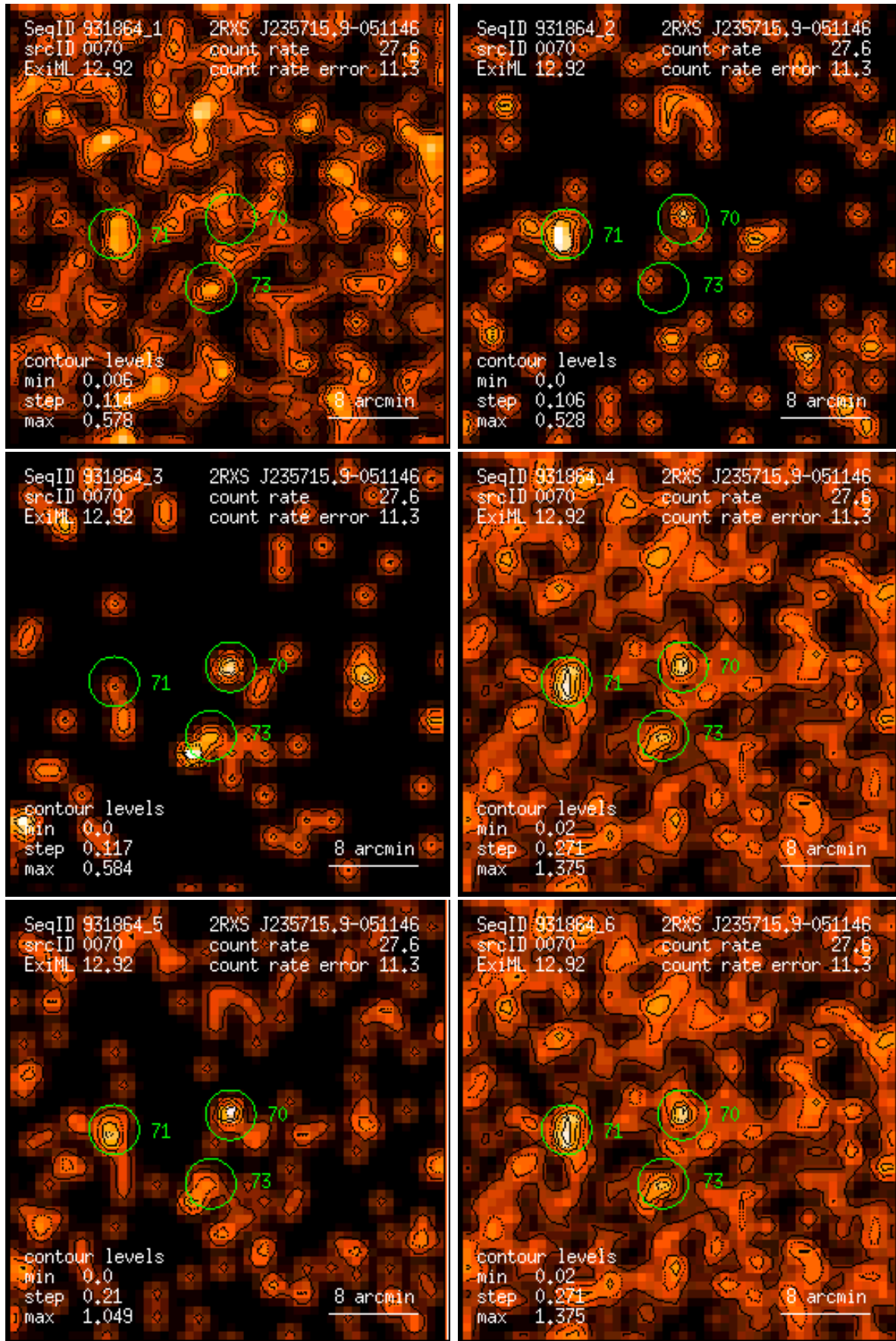
Figure 70: RASS 931864: detection 0070: band rate images, Gaussian filter: (1) PSPC channels 11 – 41, (2) 52 – 90, (3) 91 – 201, (4) 11 – 235, (5) 52 – 201, (6) 11 – 201. Broad band rates in counts/ks. Band rate contour levels in counts/ks/arcmin 2 .
