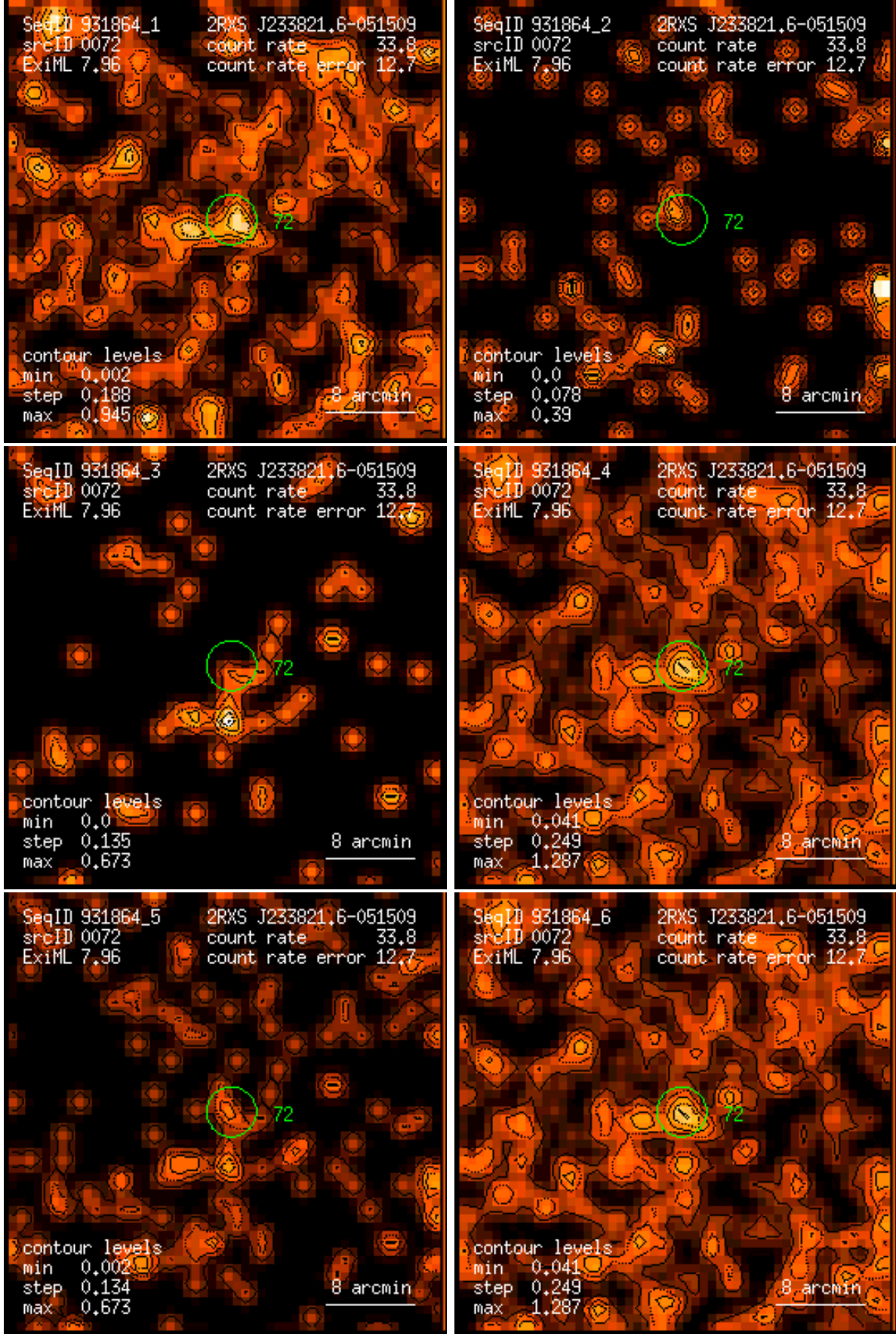
Figure 72: RASS 931864: detection 0072: band rate images, Gaussian filter: (1) PSPC channels 11 – 41, (2) 52 – 90, (3) 91 – 201, (4) 11 – 235, (5) 52 – 201, (6) 11 – 201. Broad band rates in counts/ks. Band rate contour levels in counts/ks/arcmin 2 .
