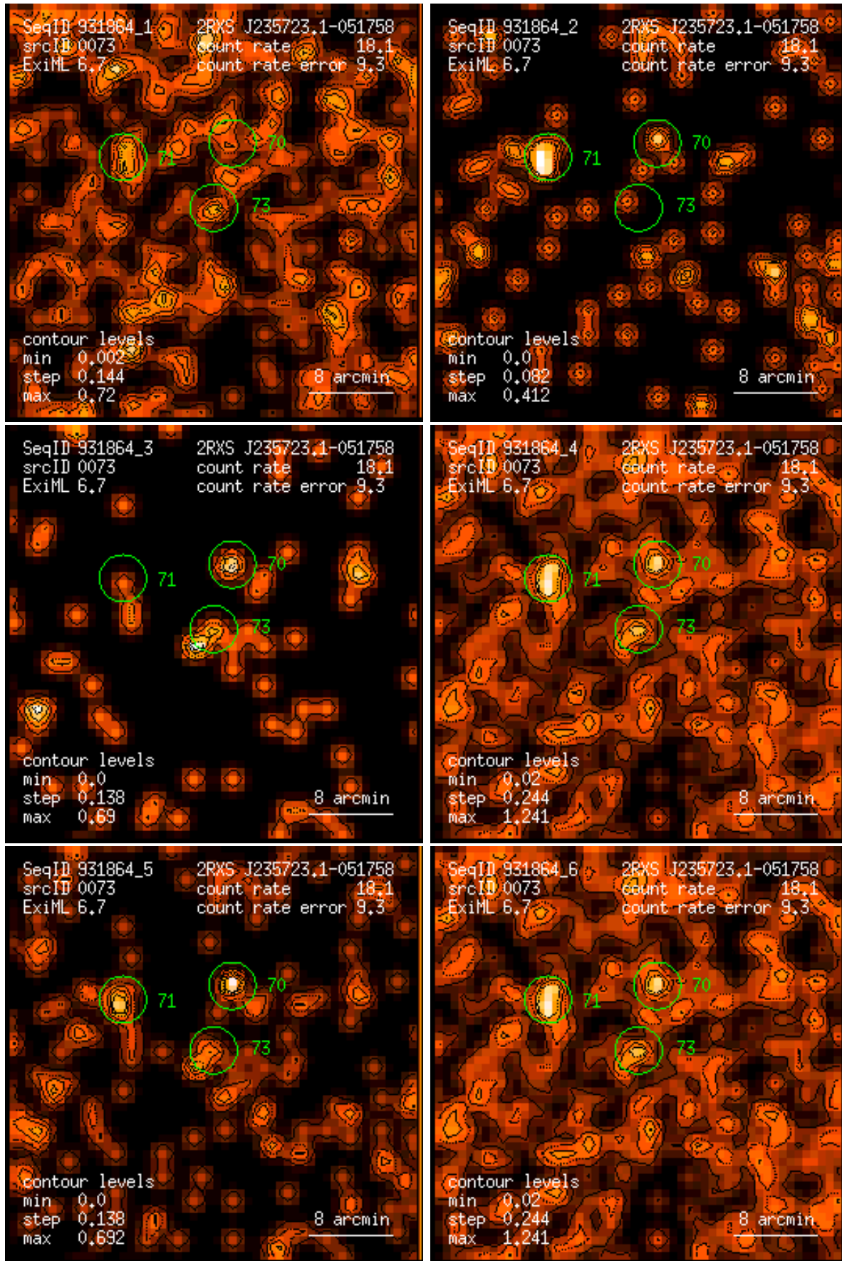
Figure 73: RASS 931864: detection 0073: band rate images, Gaussian filter: (1) PSPC channels 11 – 41, (2) 52 – 90, (3) 91 – 201, (4) 11 – 235, (5) 52 – 201, (6) 11 – 201. Broad band rates in counts/ks. Band rate contour levels in counts/ks/arcmin 2 .
