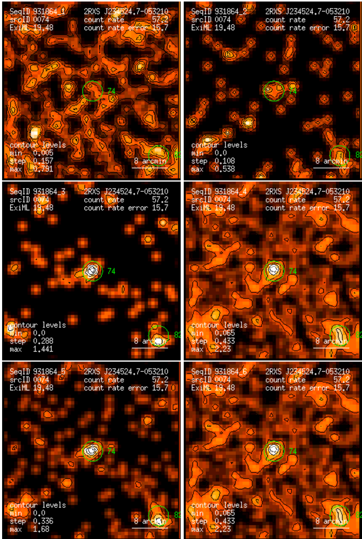
Figure 74: RASS 931864: detection 0074: band rate images, Gaussian filter: (1) PSPC channels 11 – 41, (2) 52 – 90, (3) 91 – 201, (4) 11 – 235, (5) 52 – 201, (6) 11 – 201. Broad band rates in counts/ks. Band rate contour levels in counts/ks/arcmin 2 .
