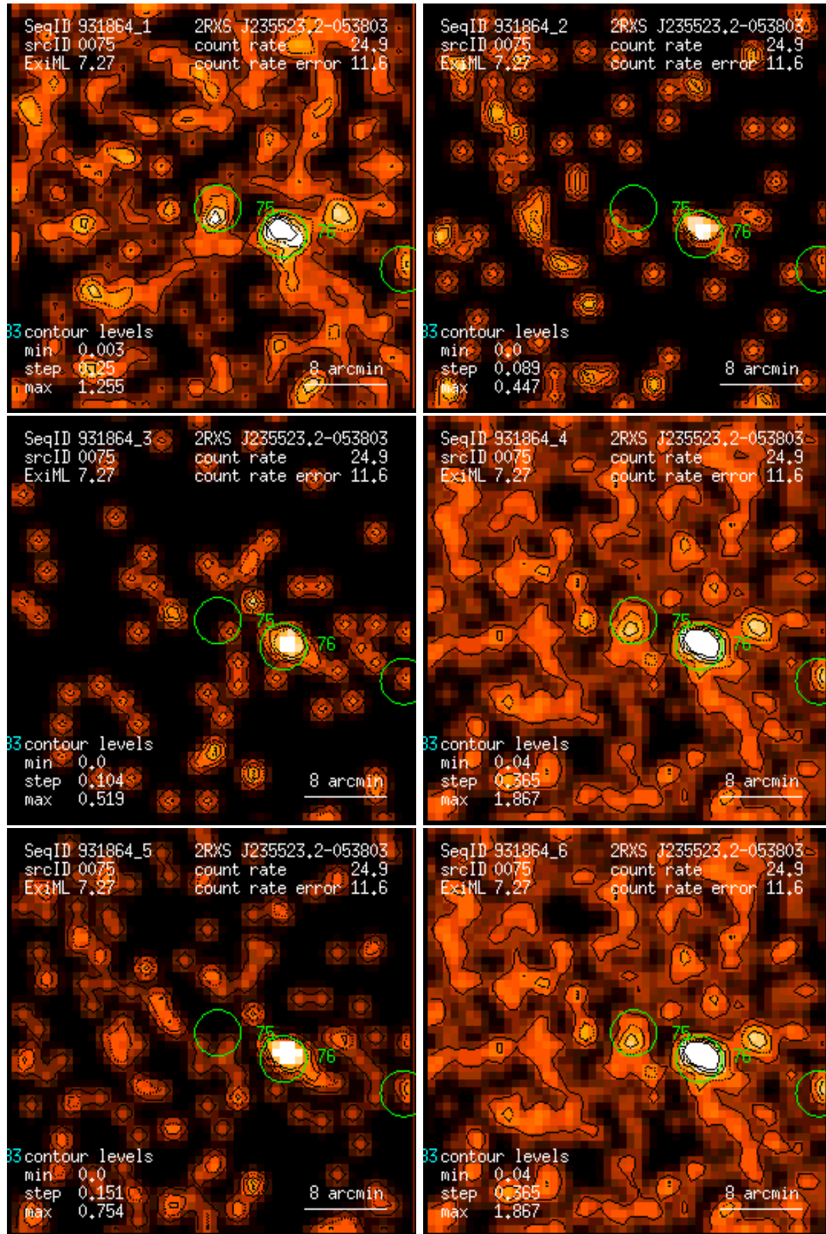
Figure 75: RASS 931864: detection 0075: band rate images, Gaussian filter: (1) PSPC channels 11 – 41, (2) 52 – 90, (3) 91 – 201, (4) 11 – 235, (5) 52 – 201, (6) 11 – 201. Broad band rates in counts/ks. Band rate contour levels in counts/ks/arcmin 2 .
