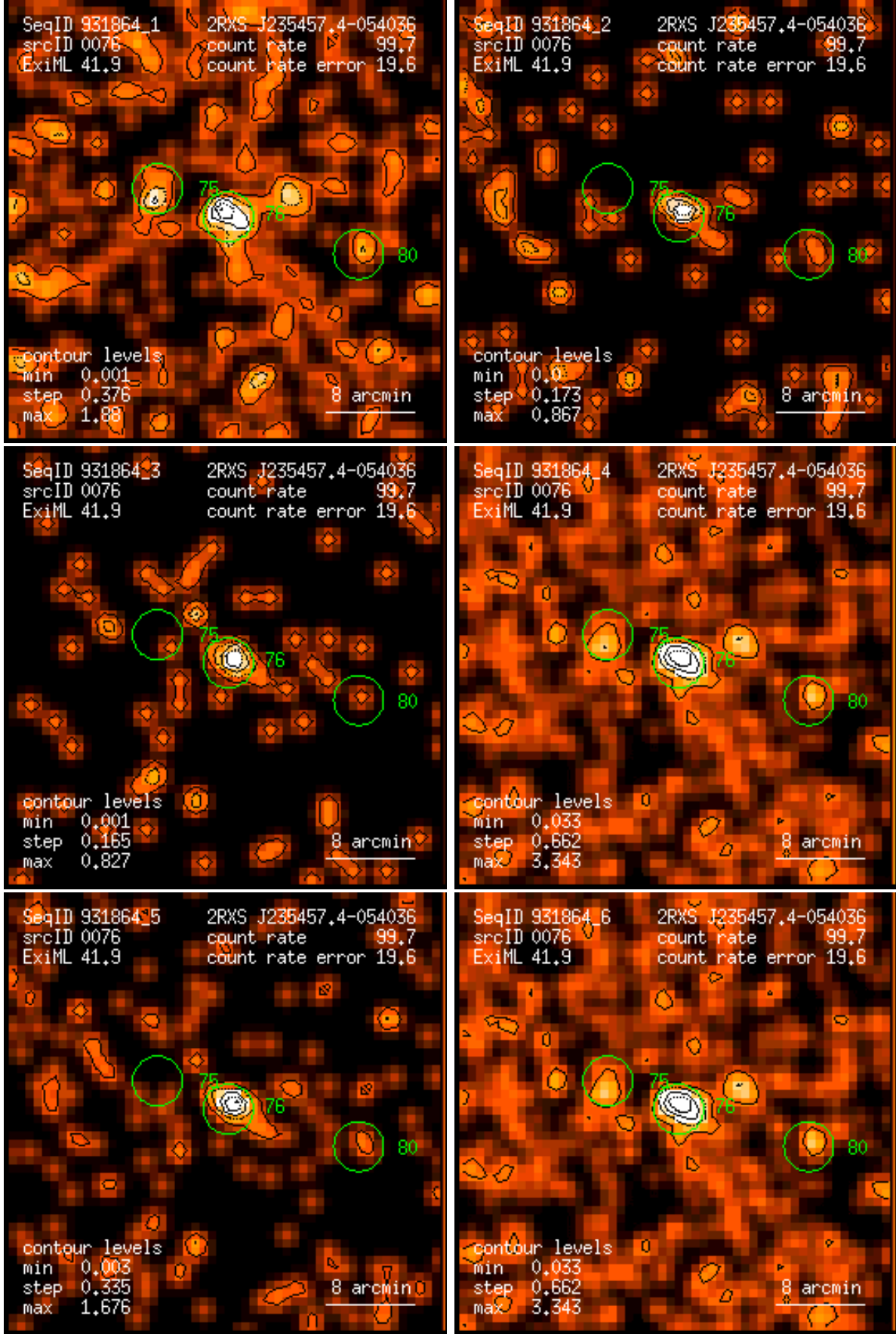
Figure 76: RASS 931864: detection 0076: band rate images, Gaussian filter: (1) PSPC channels 11 – 41, (2) 52 – 90, (3) 91 – 201, (4) 11 – 235, (5) 52 – 201, (6) 11 – 201. Broad band rates in counts/ks. Band rate contour levels in counts/ks/arcmin 2 .
