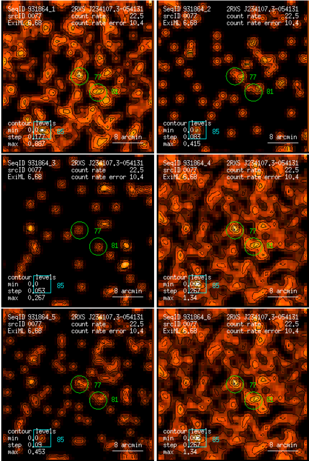
Figure 77: RASS 931864: detection 0077: band rate images, Gaussian filter: (1) PSPC channels 11 – 41, (2) 52 – 90, (3) 91 – 201, (4) 11 – 235, (5) 52 – 201, (6) 11 – 201. Broad band rates in counts/ks. Band rate contour levels in counts/ks/arcmin 2 .
