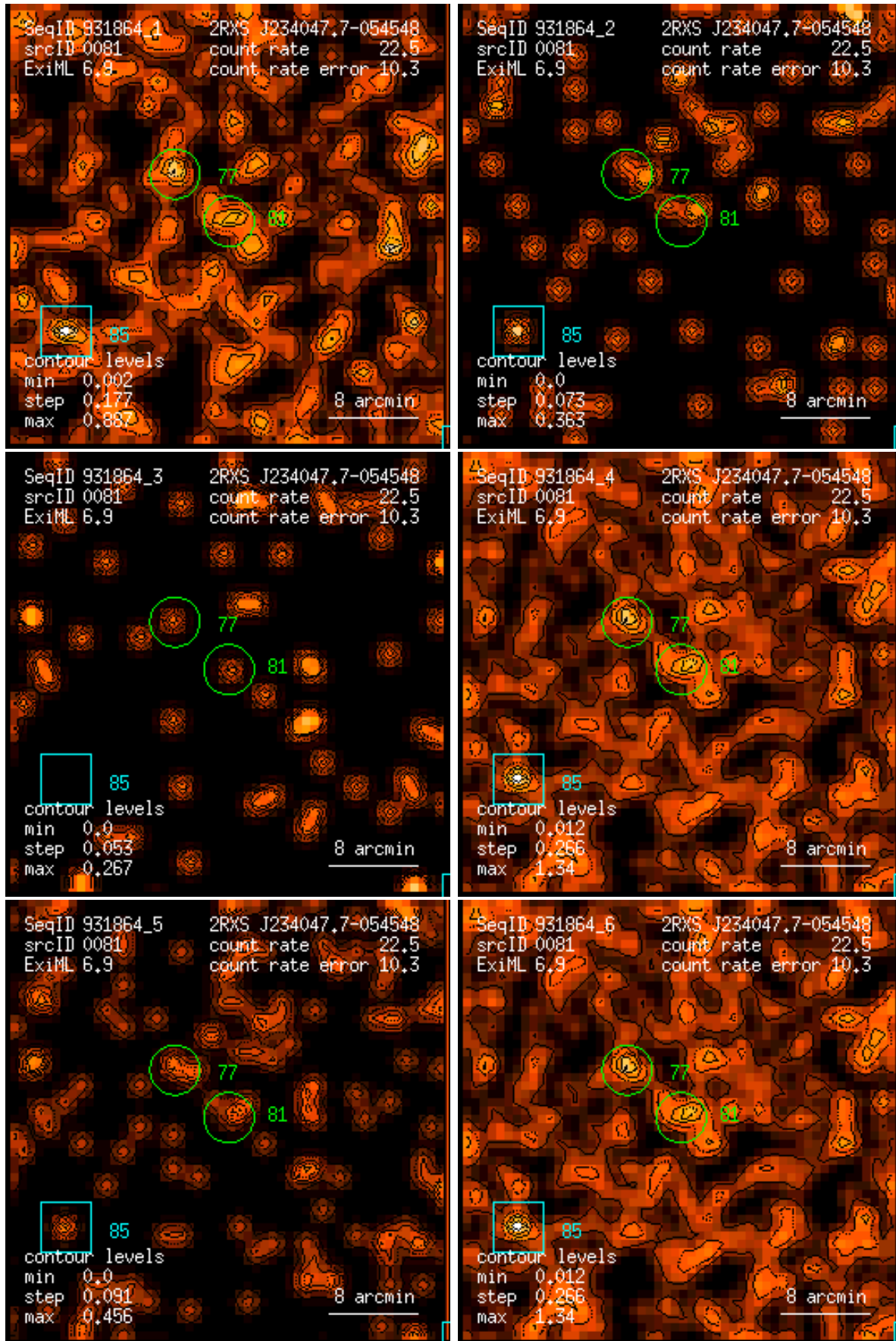
Figure 81: RASS 931864: detection 0081: band rate images, Gaussian filter: (1) PSPC channels 11 – 41, (2) 52 – 90, (3) 91 – 201, (4) 11 – 235, (5) 52 – 201, (6) 11 – 201. Broad band rates in counts/ks. Band rate contour levels in counts/ks/arcmin 2 .
