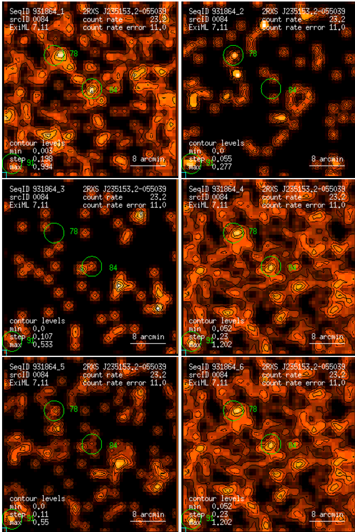
Figure 84: RASS 931864: detection 0084: band rate images, Gaussian filter: (1) PSPC channels 11 – 41, (2) 52 – 90, (3) 91 – 201, (4) 11 – 235, (5) 52 – 201, (6) 11 – 201. Broad band rates in counts/ks. Band rate contour levels in counts/ks/arcmin 2 .
