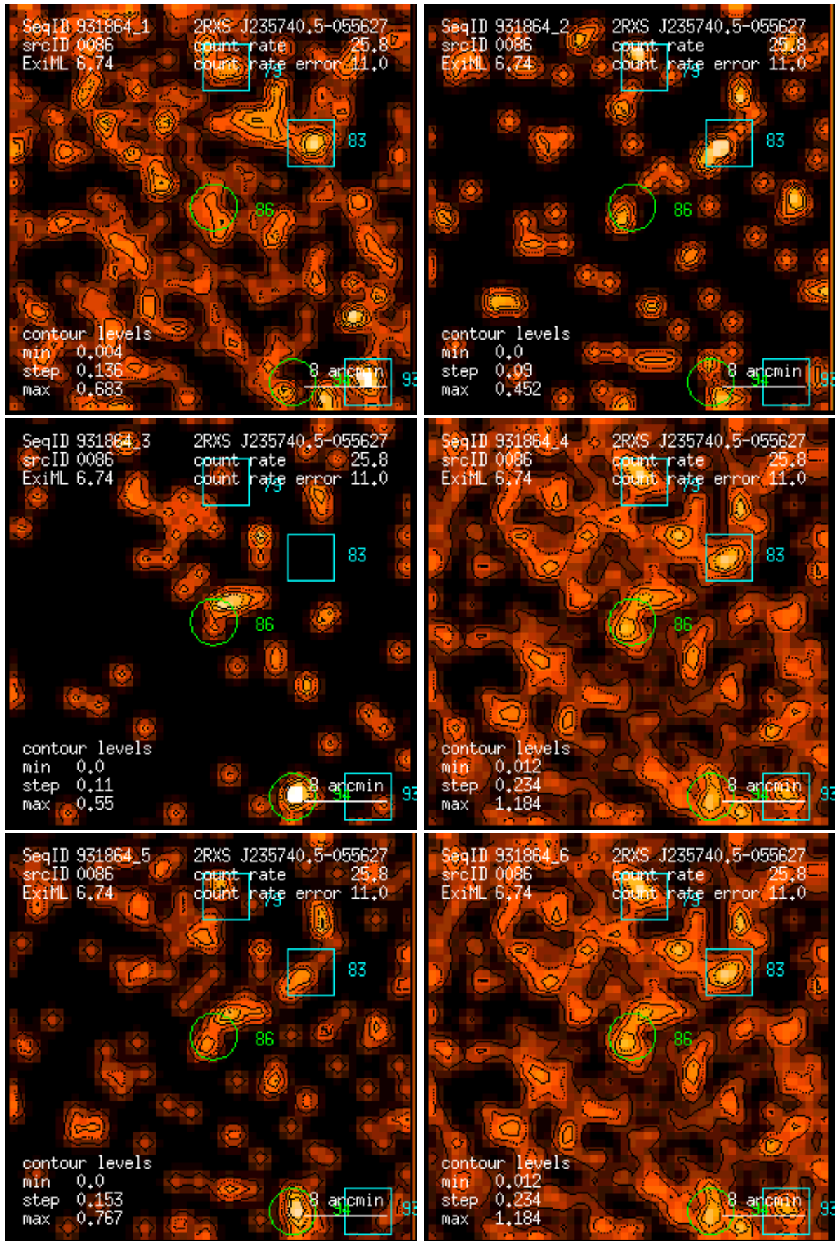
Figure 86: RASS 931864: detection 0086: band rate images, Gaussian filter: (1) PSPC channels 11 – 41, (2) 52 – 90, (3) 91 – 201, (4) 11 – 235, (5) 52 – 201, (6) 11 – 201. Broad band rates in counts/ks. Band rate contour levels in counts/ks/arcmin 2 .
