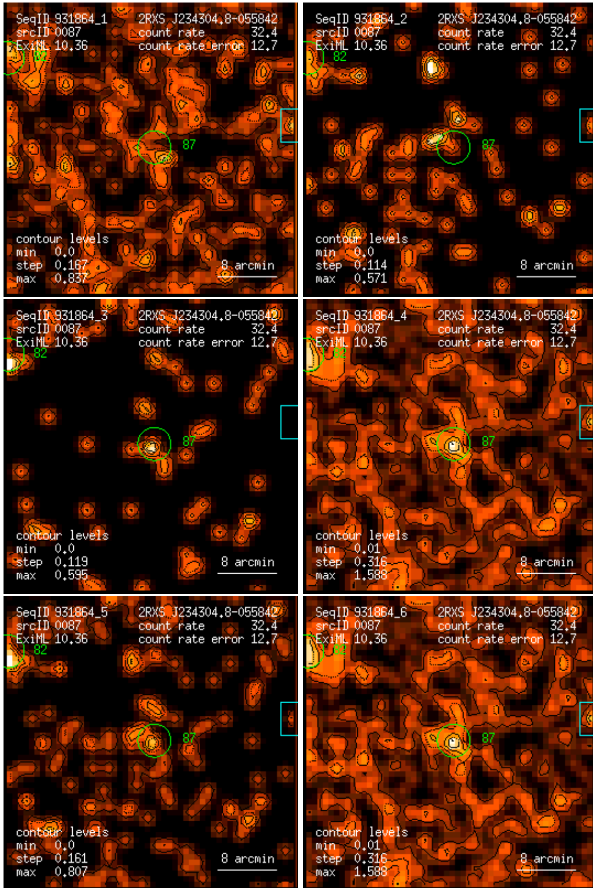
Figure 87: RASS 931864: detection 0087: band rate images, Gaussian filter: (1) PSPC channels 11 – 41, (2) 52 – 90, (3) 91 – 201, (4) 11 – 235, (5) 52 – 201, (6) 11 – 201. Broad band rates in counts/ks. Band rate contour levels in counts/ks/arcmin 2 .
