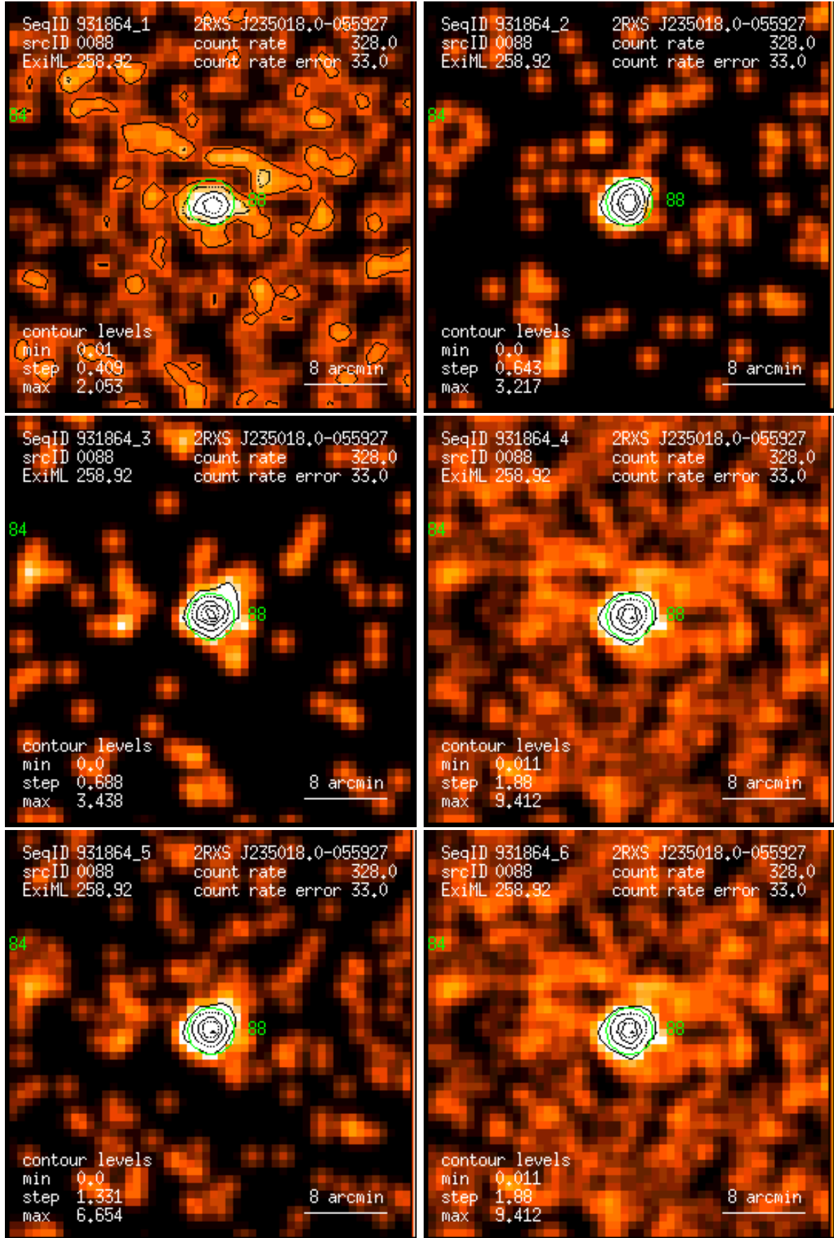
Figure 88: RASS 931864: detection 0088: band rate images, Gaussian filter: (1) PSPC channels 11 – 41, (2) 52 – 90, (3) 91 – 201, (4) 11 – 235, (5) 52 – 201, (6) 11 – 201. Broad band rates in counts/ks. Band rate contour levels in counts/ks/arcmin 2 .
