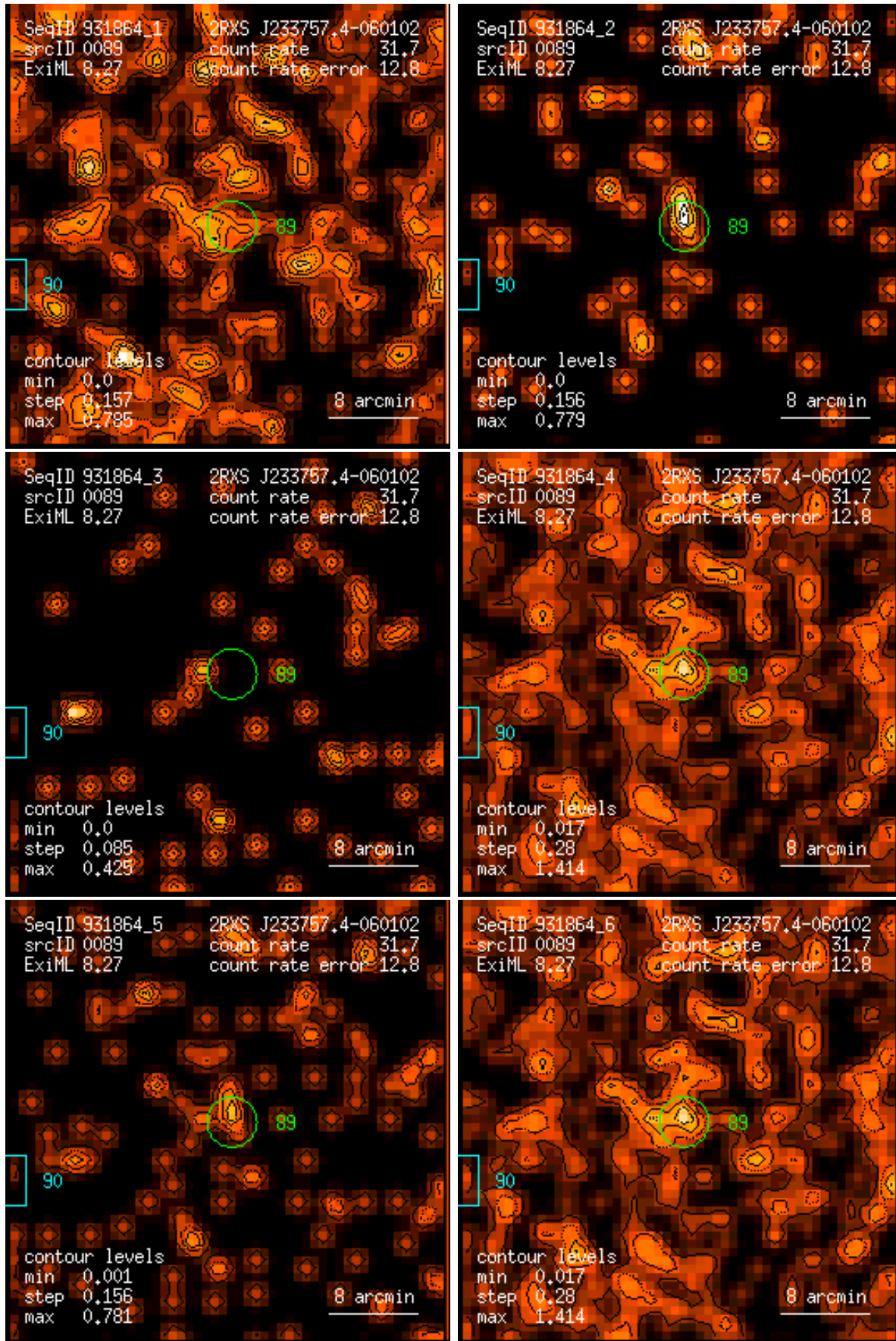
Figure 89: RASS 931864: detection 0089: band rate images, Gaussian filter: (1) PSPC channels 11 – 41, (2) 52 – 90, (3) 91 – 201, (4) 11 – 235, (5) 52 – 201, (6) 11 – 201. Broad band rates in counts/ks. Band rate contour levels in counts/ks/arcmin 2 .
