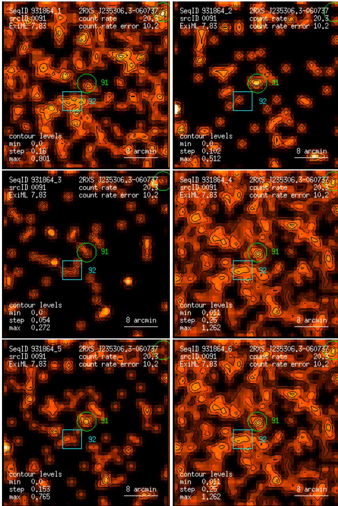
Figure 91: RASS 931864: detection 0091: band rate images, Gaussian filter: (1) PSPC channels 11 – 41, (2) 52 – 90, (3) 91 – 201, (4) 11 – 235, (5) 52 – 201, (6) 11 – 201. Broad band rates in counts/ks. Band rate contour levels in counts/ks/arcmin 2 .
