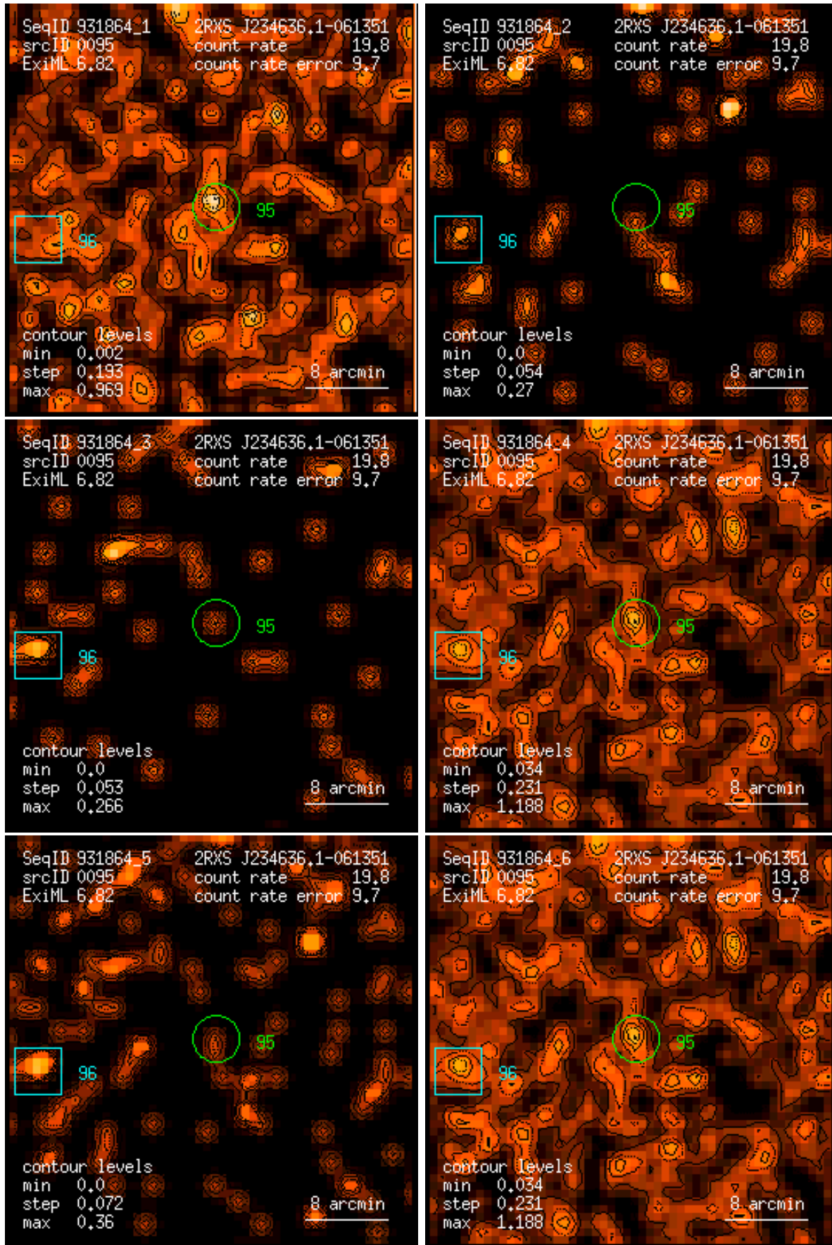
Figure 95: RASS 931864: detection 0095: band rate images, Gaussian filter: (1) PSPC channels 11 – 41, (2) 52 – 90, (3) 91 – 201, (4) 11 – 235, (5) 52 – 201, (6) 11 – 201. Broad band rates in counts/ks. Band rate contour levels in counts/ks/arcmin 2 .
