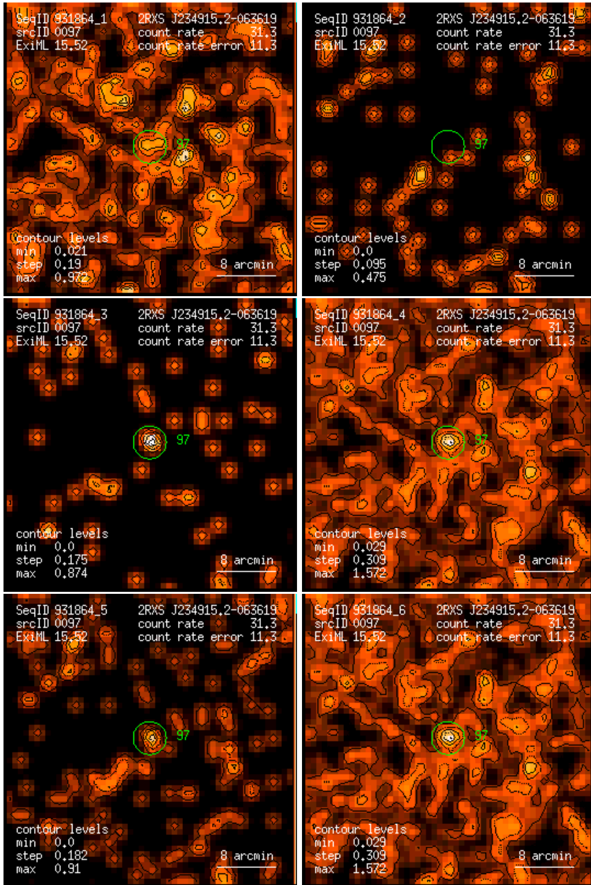
Figure 97: RASS 931864: detection 0097: band rate images, Gaussian filter: (1) PSPC channels 11 – 41, (2) 52 – 90, (3) 91 – 201, (4) 11 – 235, (5) 52 – 201, (6) 11 – 201. Broad band rates in counts/ks. Band rate contour levels in counts/ks/arcmin 2 .
