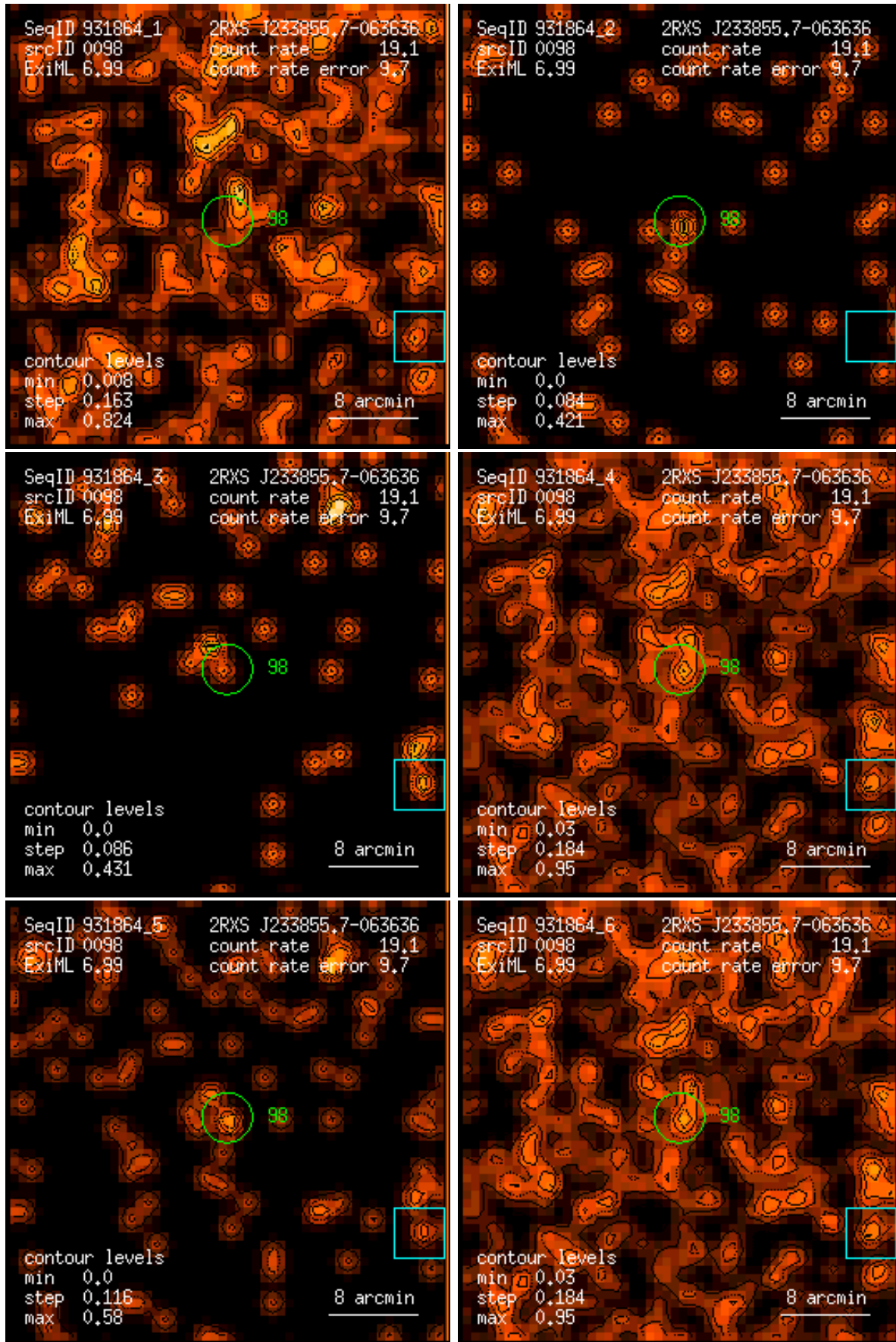
Figure 98: RASS 931864: detection 0098: band rate images, Gaussian filter: (1) PSPC channels 11 – 41, (2) 52 – 90, (3) 91 – 201, (4) 11 – 235, (5) 52 – 201, (6) 11 – 201. Broad band rates in counts/ks. Band rate contour levels in counts/ks/arcmin 2 .
