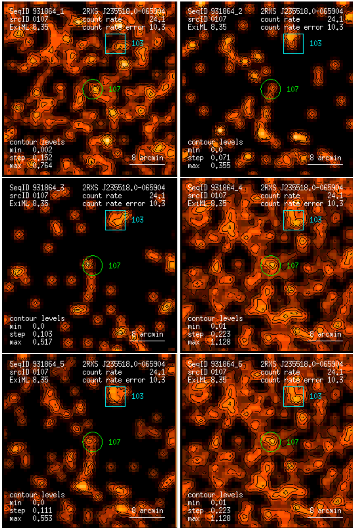
Figure 107: RASS 931864: detection 0107: band rate images, Gaussian filter: (1) PSPC channels 11 – 41, (2) 52 – 90, (3) 91 – 201, (4) 11 – 235, (5) 52 – 201, (6) 11 – 201. Broad band rates in counts/ks. Band rate contour levels in counts/ks/arcmin 2 .
