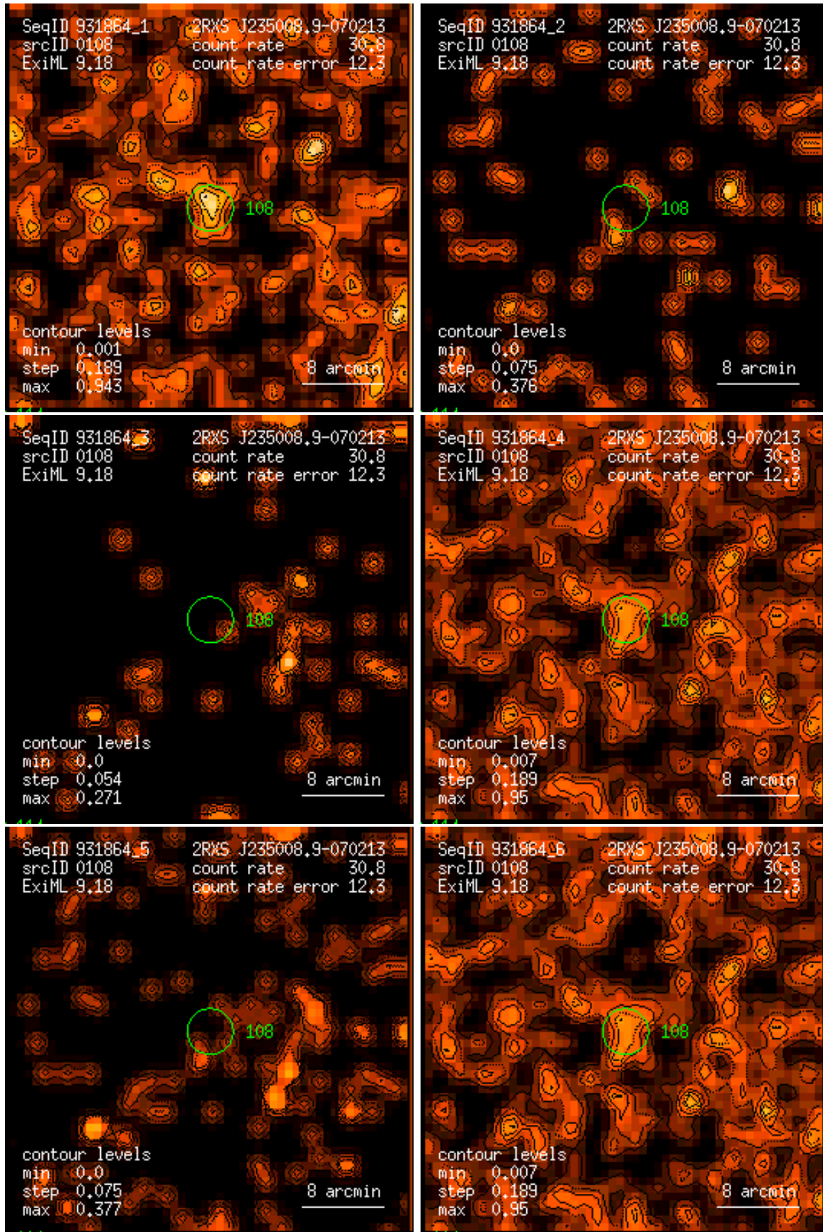
Figure 108: RASS 931864: detection 0108: band rate images, Gaussian filter: (1) PSPC channels 11 – 41, (2) 52 – 90, (3) 91 – 201, (4) 11 – 235, (5) 52 – 201, (6) 11 – 201. Broad band rates in counts/ks. Band rate contour levels in counts/ks/arcmin 2 .
