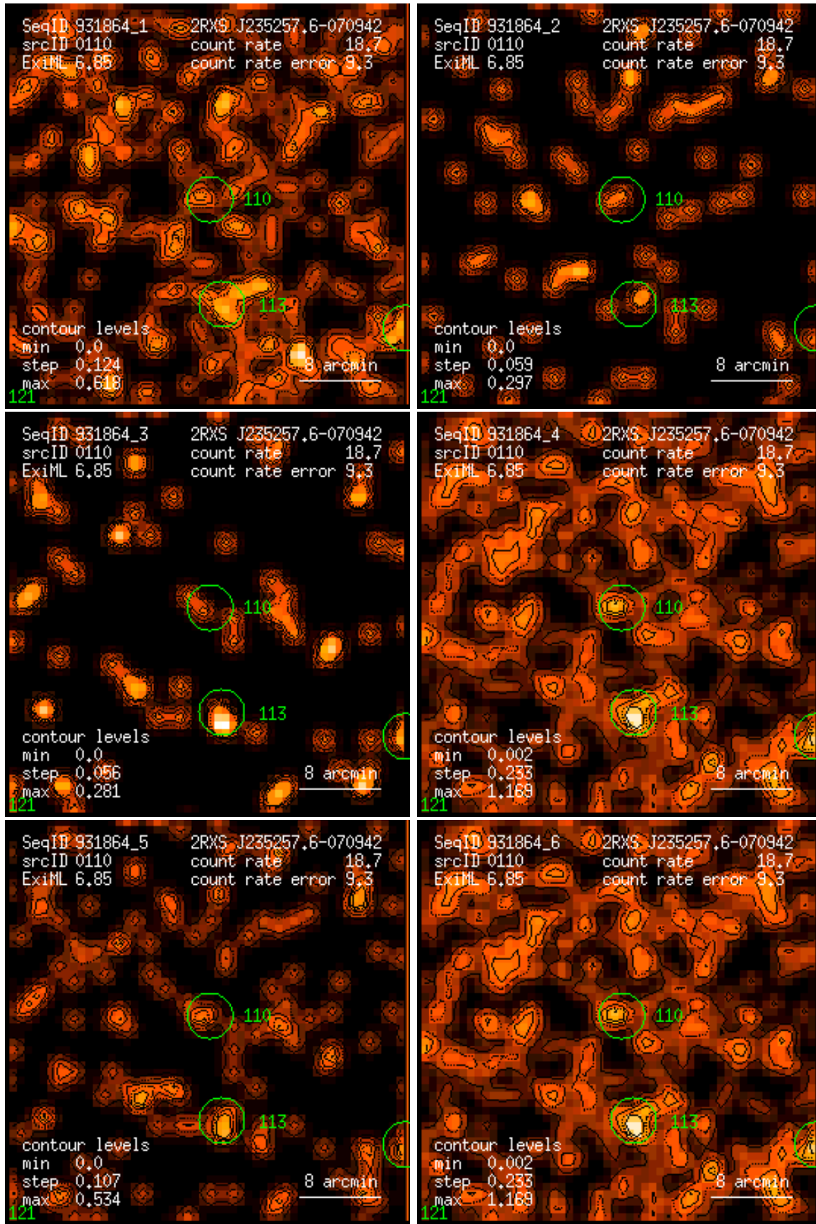
Figure 110: RASS 931864: detection 0110: band rate images, Gaussian filter: (1) PSPC channels 11 – 41, (2) 52 – 90, (3) 91 – 201, (4) 11 – 235, (5) 52 – 201, (6) 11 – 201. Broad band rates in counts/ks. Band rate contour levels in counts/ks/arcmin 2 .
