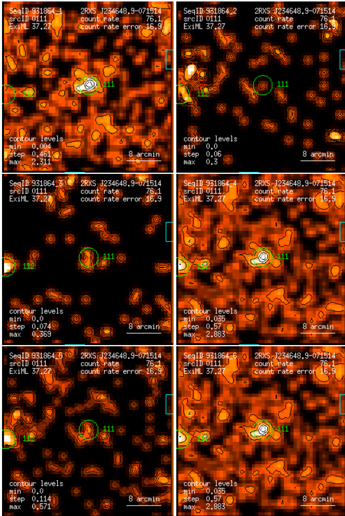
Figure 111: RASS 931864: detection 0111: band rate images, Gaussian filter: (1) PSPC channels 11 – 41, (2) 52 – 90, (3) 91 – 201, (4) 11 – 235, (5) 52 – 201, (6) 11 – 201. Broad band rates in counts/ks. Band rate contour levels in counts/ks/arcmin 2 .
