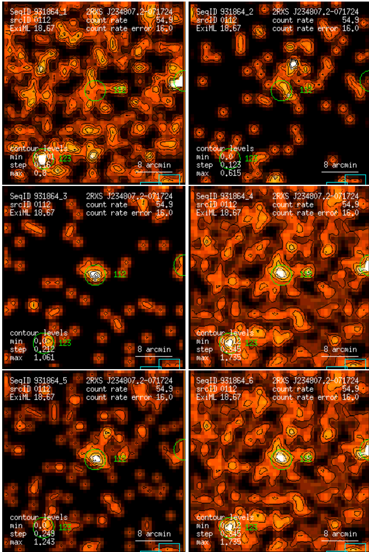
Figure 112: RASS 931864: detection 0112: band rate images, Gaussian filter: (1) PSPC channels 11 – 41, (2) 52 – 90, (3) 91 – 201, (4) 11 – 235, (5) 52 – 201, (6) 11 – 201. Broad band rates in counts/ks. Band rate contour levels in counts/ks/arcmin 2 .
