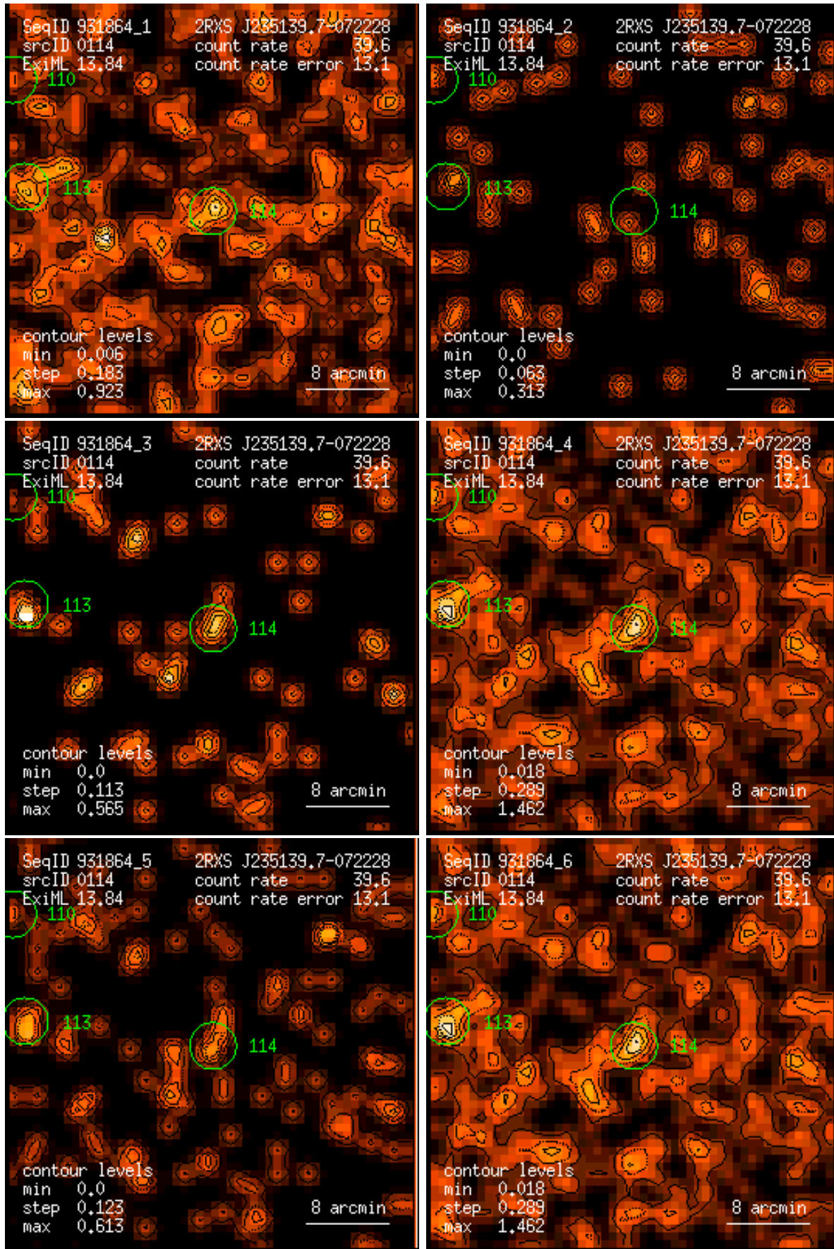
Figure 114: RASS 931864: detection 0114: band rate images, Gaussian filter: (1) PSPC channels 11 – 41, (2) 52 – 90, (3) 91 – 201, (4) 11 – 235, (5) 52 – 201, (6) 11 – 201. Broad band rates in counts/ks. Band rate contour levels in counts/ks/arcmin 2 .
