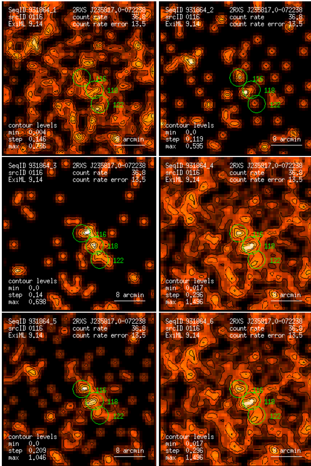
Figure 116: RASS 931864: detection 0116: band rate images, Gaussian filter: (1) PSPC channels 11 – 41, (2) 52 – 90, (3) 91 – 201, (4) 11 – 235, (5) 52 – 201, (6) 11 – 201. Broad band rates in counts/ks. Band rate contour levels in counts/ks/arcmin 2 .
