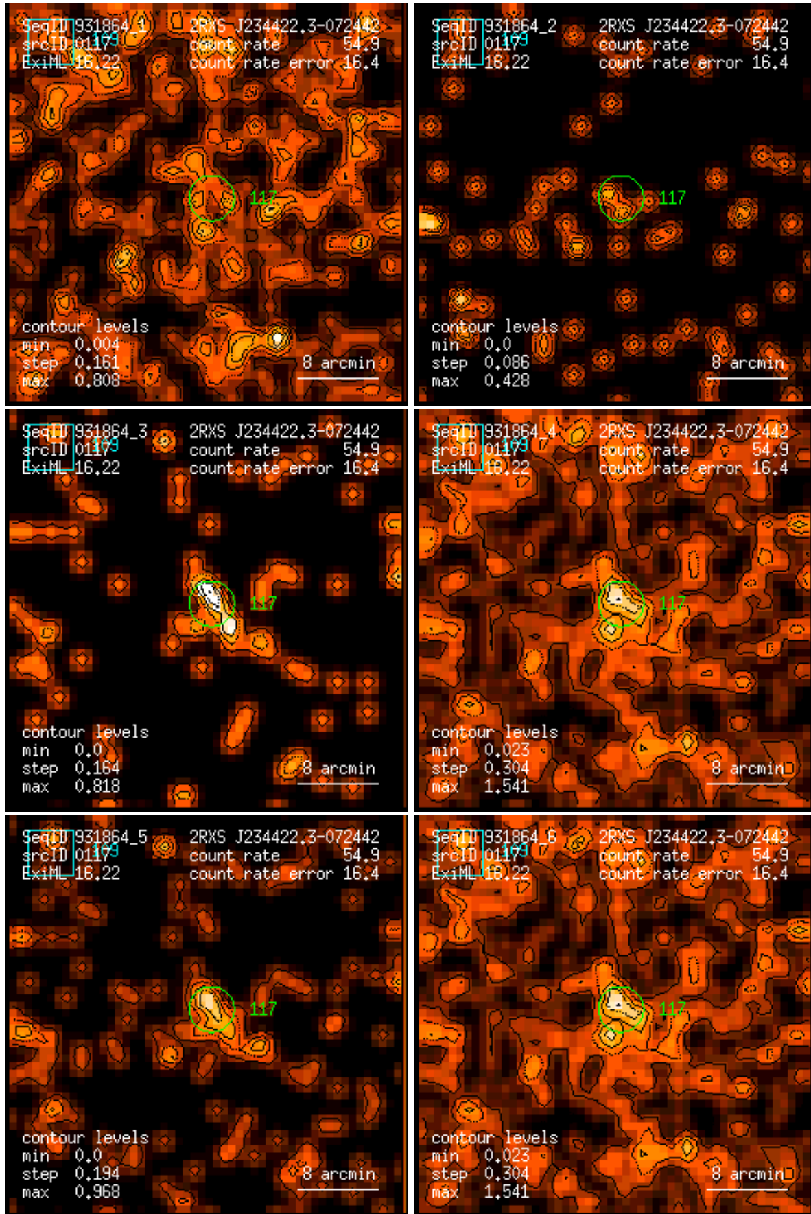
Figure 117: RASS 931864: detection 0117: band rate images, Gaussian filter: (1) PSPC channels 11 – 41, (2) 52 – 90, (3) 91 – 201, (4) 11 – 235, (5) 52 – 201, (6) 11 – 201. Broad band rates in counts/ks. Band rate contour levels in counts/ks/arcmin 2 .
