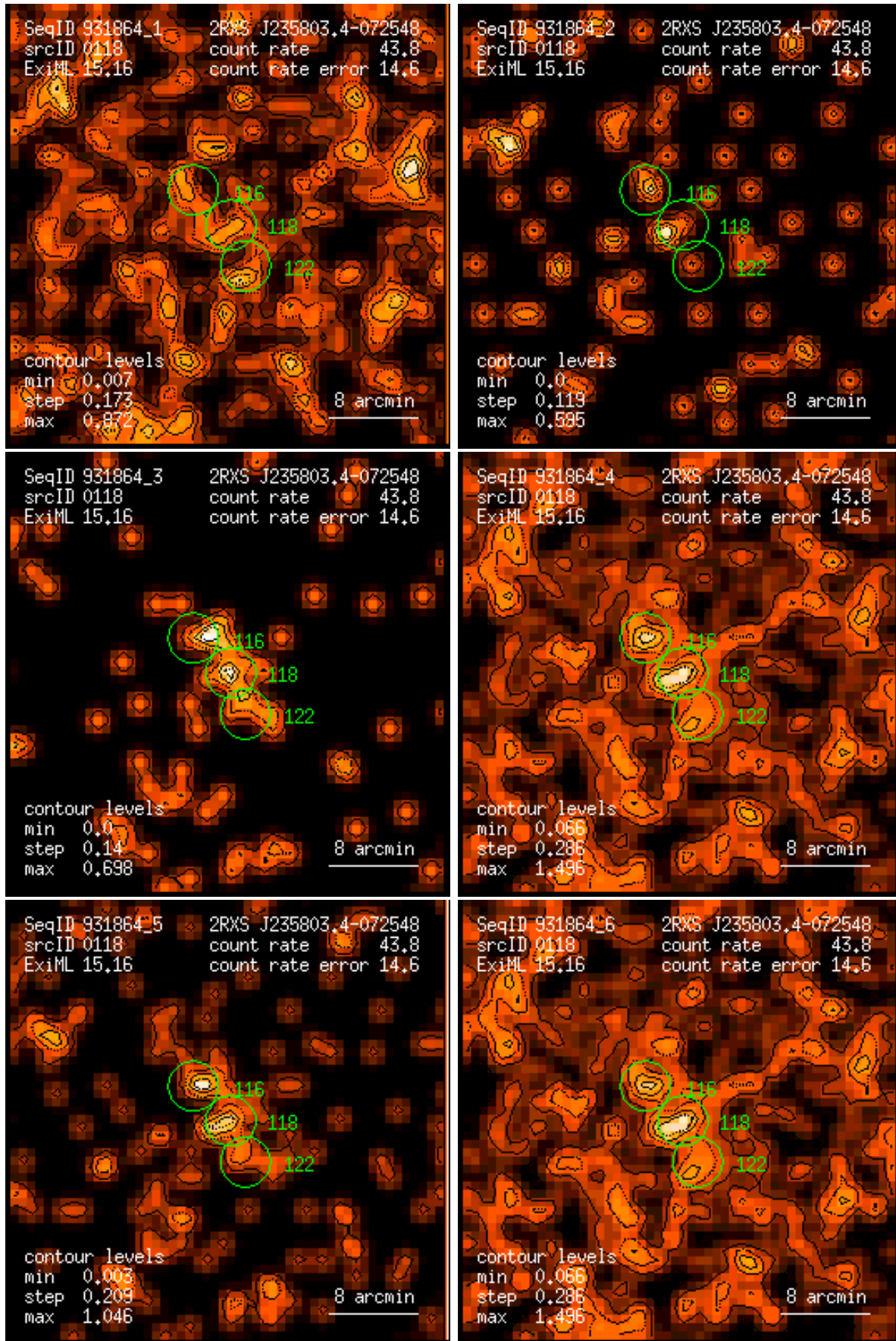
Figure 118: RASS 931864: detection 0118: band rate images, Gaussian filter: (1) PSPC channels 11 – 41, (2) 52 – 90, (3) 91 – 201, (4) 11 – 235, (5) 52 – 201, (6) 11 – 201. Broad band rates in counts/ks. Band rate contour levels in counts/ks/arcmin 2 .
