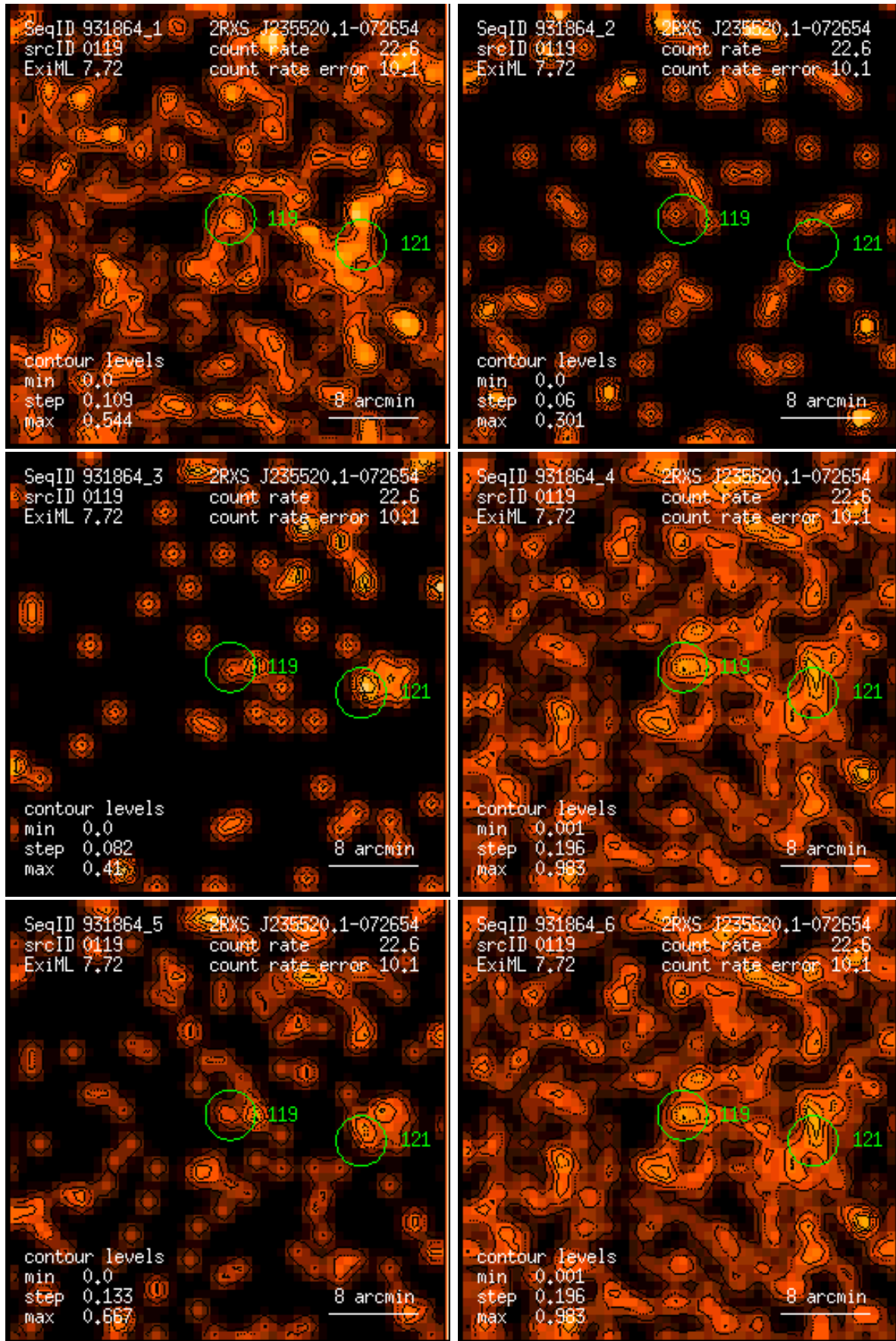
Figure 119: RASS 931864: detection 0119: band rate images, Gaussian filter: (1) PSPC channels 11 – 41, (2) 52 – 90, (3) 91 – 201, (4) 11 – 235, (5) 52 – 201, (6) 11 – 201. Broad band rates in counts/ks. Band rate contour levels in counts/ks/arcmin 2 .
