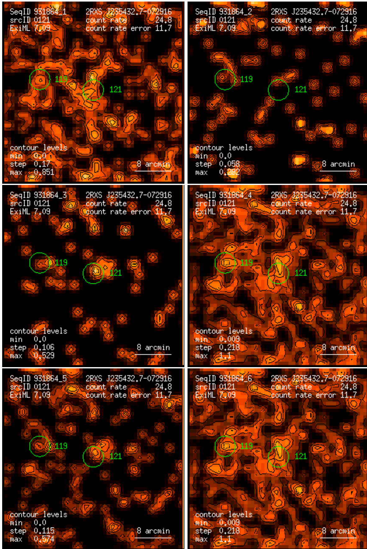
Figure 121: RASS 931864: detection 0121: band rate images, Gaussian filter: (1) PSPC channels 11 – 41, (2) 52 – 90, (3) 91 – 201, (4) 11 – 235, (5) 52 – 201, (6) 11 – 201. Broad band rates in counts/ks. Band rate contour levels in counts/ks/arcmin 2 .
