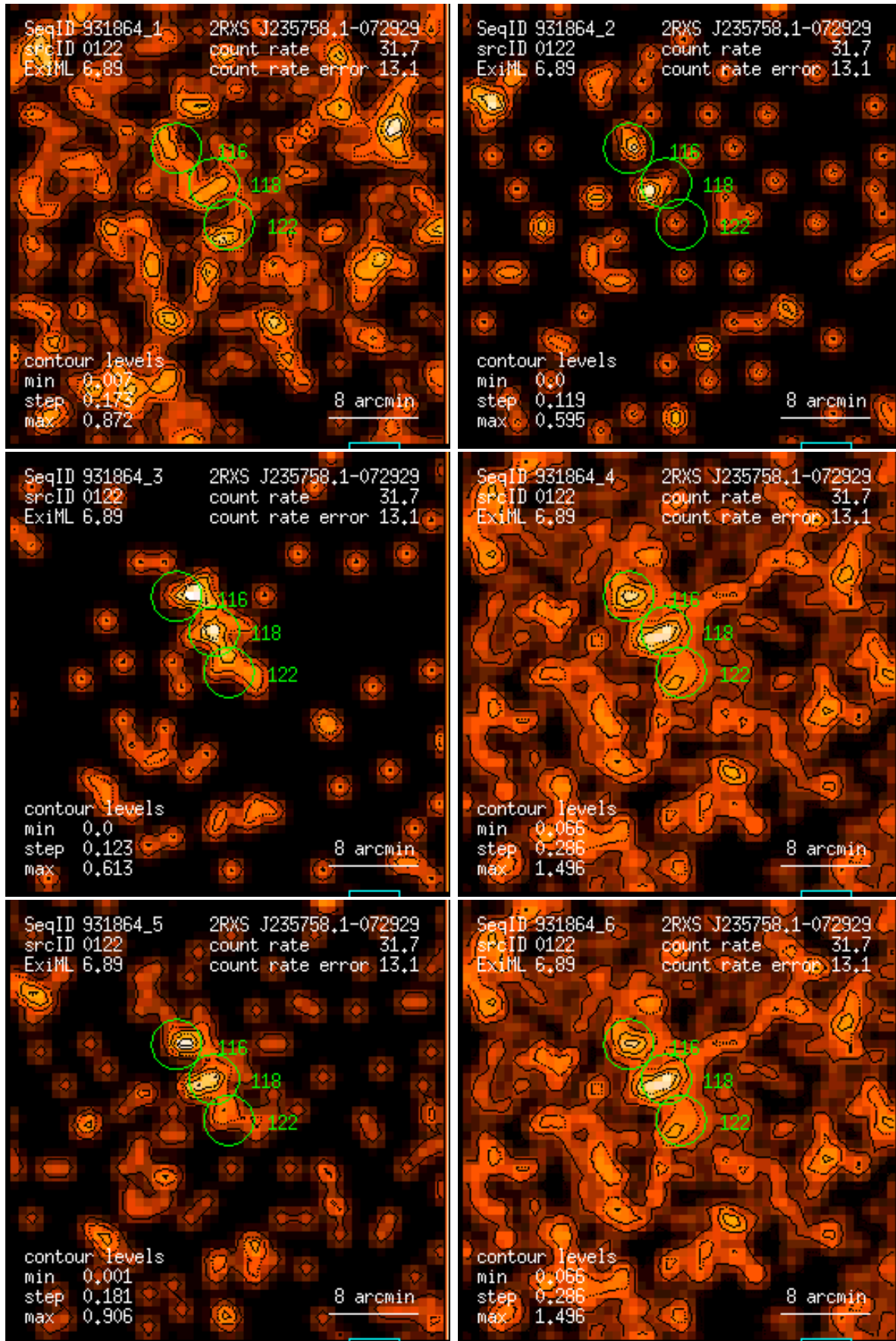
Figure 122: RASS 931864: detection 0122: band rate images, Gaussian filter: (1) PSPC channels 11 – 41, (2) 52 – 90, (3) 91 – 201, (4) 11 – 235, (5) 52 – 201, (6) 11 – 201. Broad band rates in counts/ks. Band rate contour levels in counts/ks/arcmin 2 .
