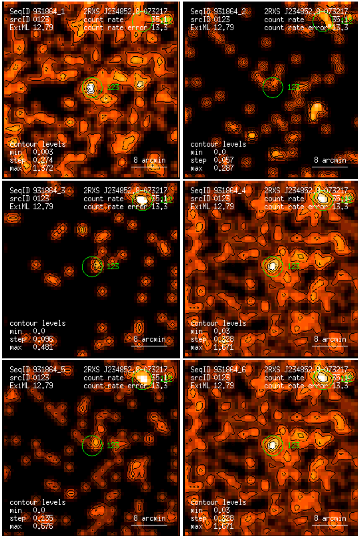
Figure 123: RASS 931864: detection 0123: band rate images, Gaussian filter: (1) PSPC channels 11 – 41, (2) 52 – 90, (3) 91 – 201, (4) 11 – 235, (5) 52 – 201, (6) 11 – 201. Broad band rates in counts/ks. Band rate contour levels in counts/ks/arcmin 2 .
