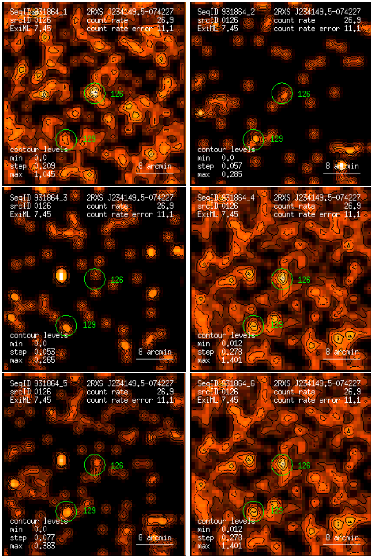
Figure 126: RASS 931864: detection 0126: band rate images, Gaussian filter: (1) PSPC channels 11 – 41, (2) 52 – 90, (3) 91 – 201, (4) 11 – 235, (5) 52 – 201, (6) 11 – 201. Broad band rates in counts/ks. Band rate contour levels in counts/ks/arcmin 2 .
