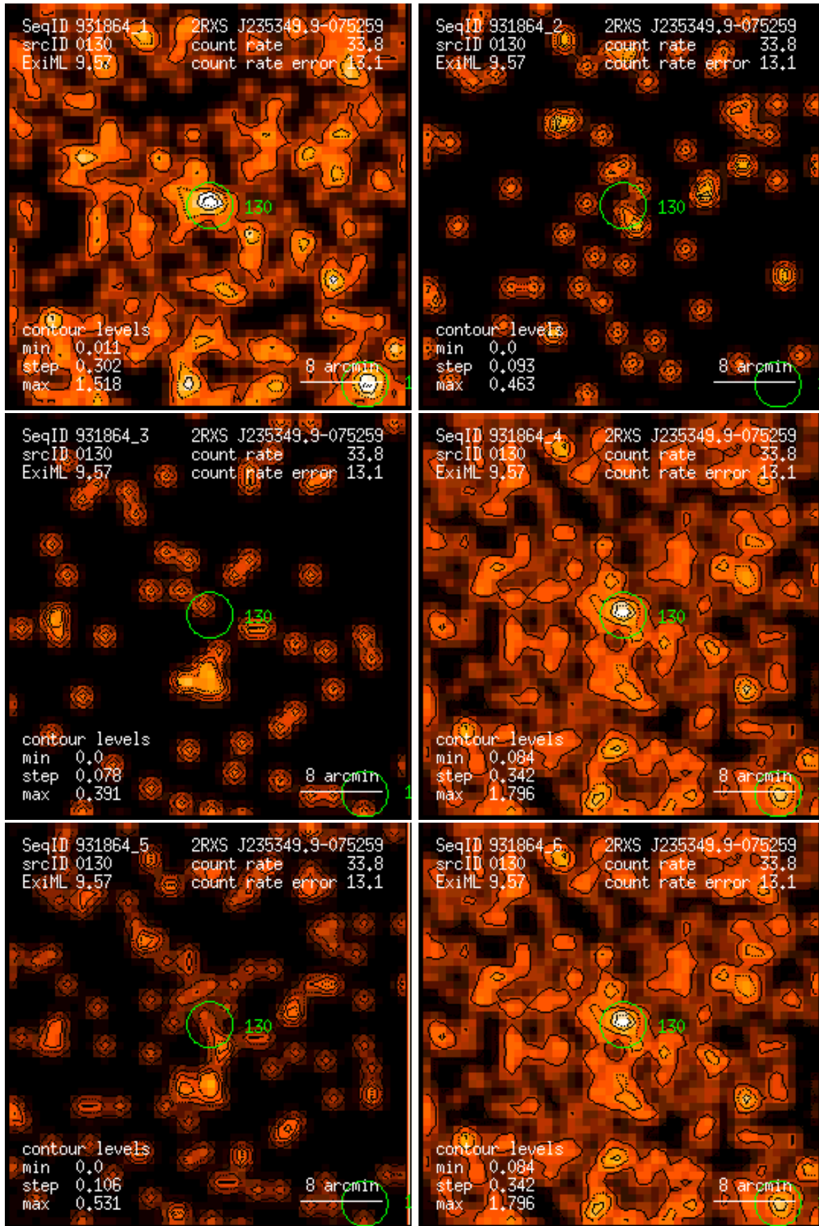
Figure 130: RASS 931864: detection 0130: band rate images, Gaussian filter: (1) PSPC channels 11 – 41, (2) 52 – 90, (3) 91 – 201, (4) 11 – 235, (5) 52 – 201, (6) 11 – 201. Broad band rates in counts/ks. Band rate contour levels in counts/ks/arcmin 2 .
