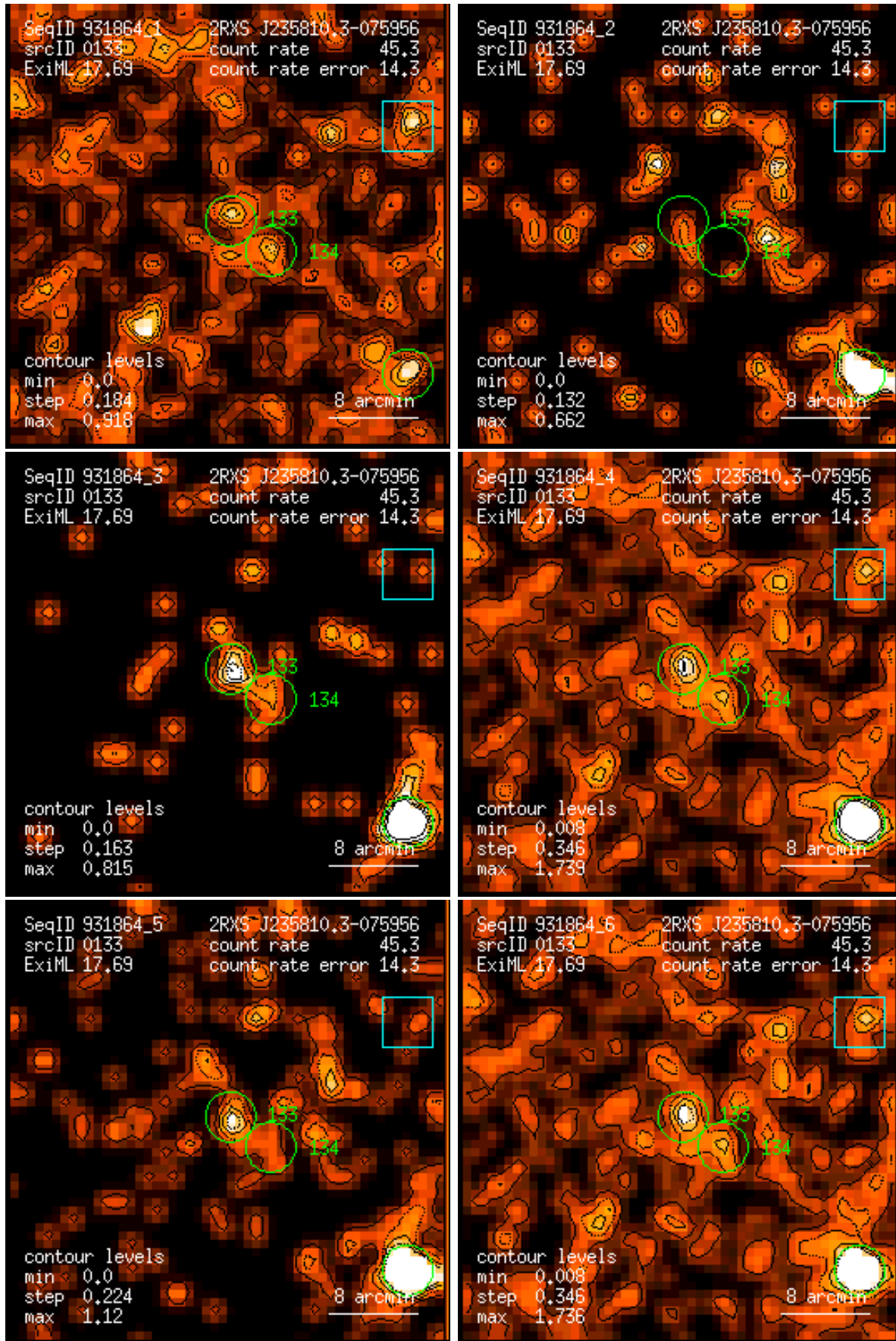
Figure 133: RASS 931864: detection 0133: band rate images, Gaussian filter: (1) PSPC channels 11 – 41, (2) 52 – 90, (3) 91 – 201, (4) 11 – 235, (5) 52 – 201, (6) 11 – 201. Broad band rates in counts/ks. Band rate contour levels in counts/ks/arcmin 2 .
