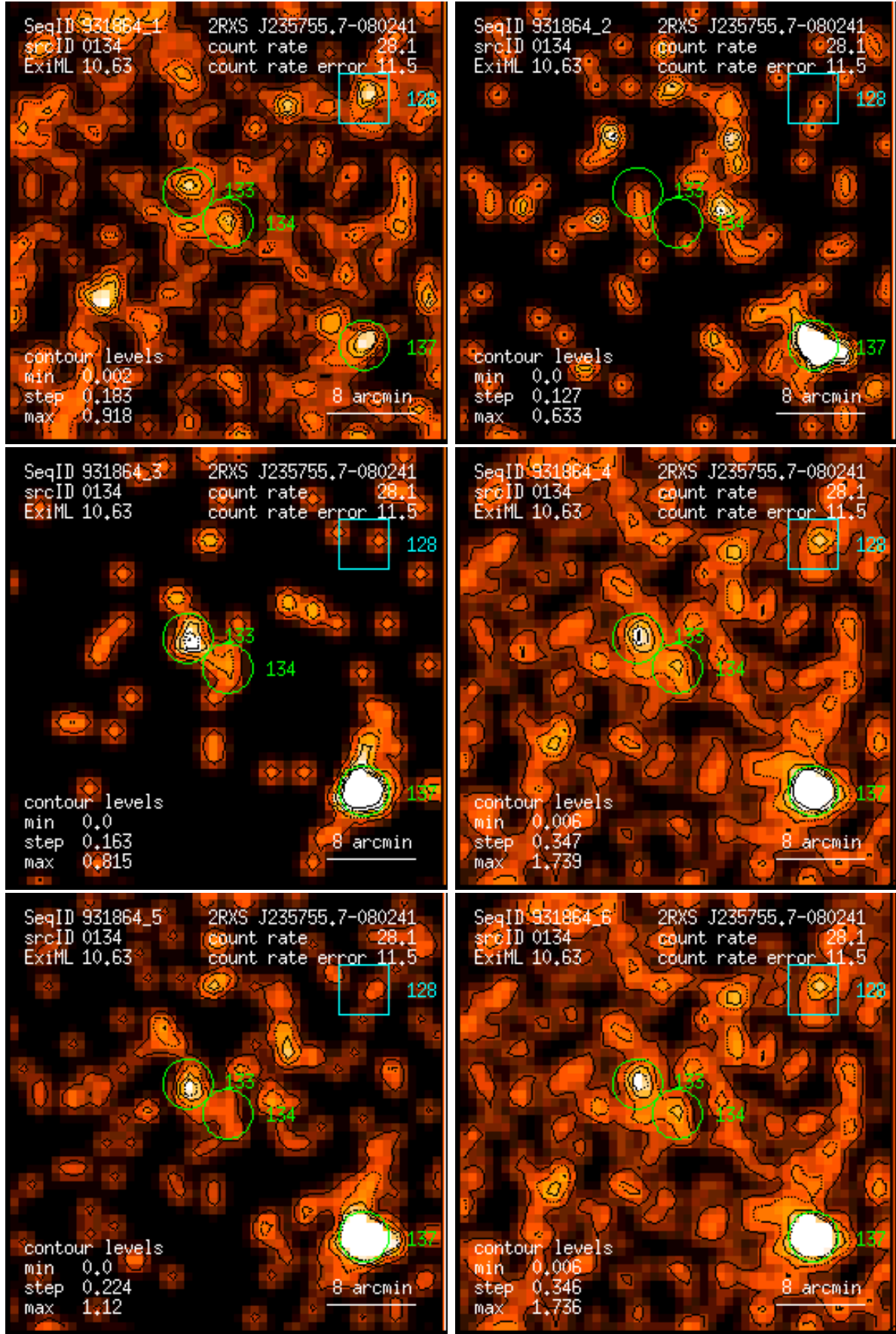
Figure 134: RASS 931864: detection 0134: band rate images, Gaussian filter: (1) PSPC channels 11 – 41, (2) 52 – 90, (3) 91 – 201, (4) 11 – 235, (5) 52 – 201, (6) 11 – 201. Broad band rates in counts/ks. Band rate contour levels in counts/ks/arcmin 2 .
