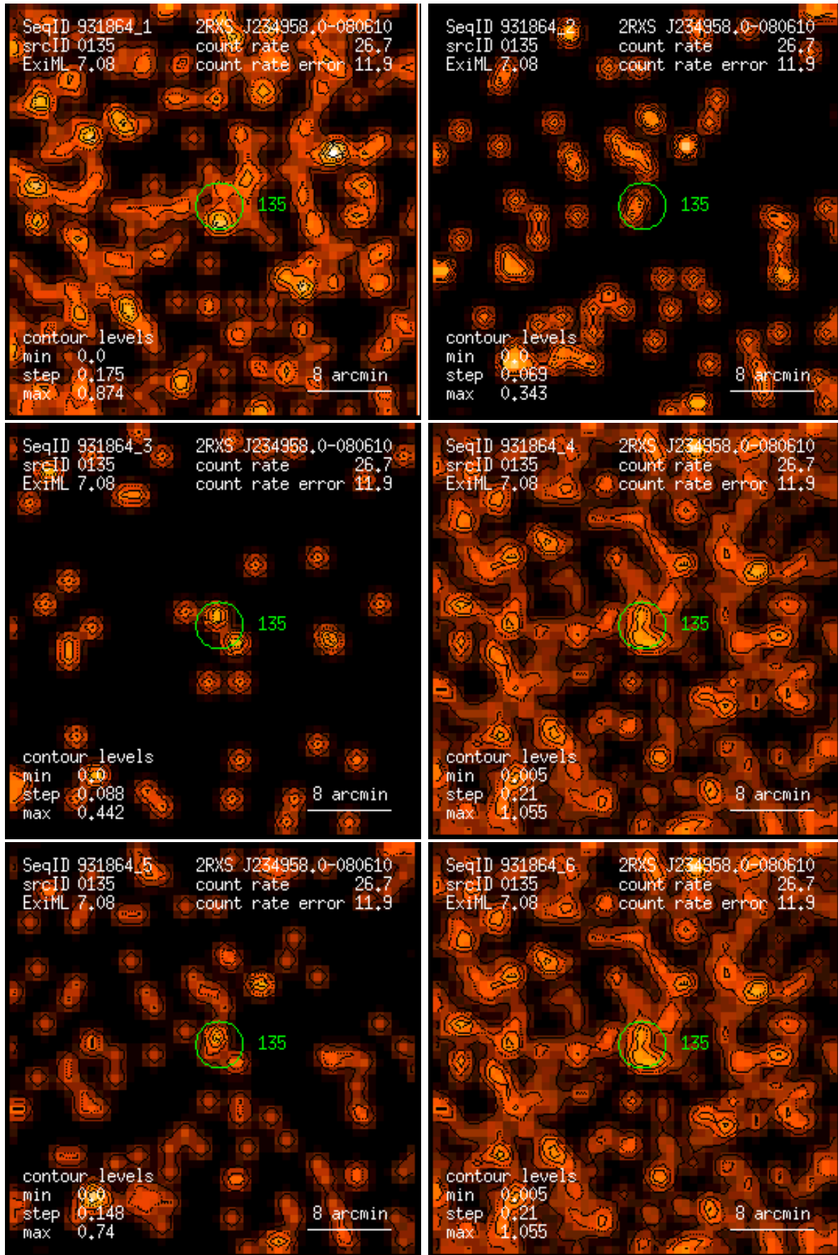
Figure 135: RASS 931864: detection 0135: band rate images, Gaussian filter: (1) PSPC channels 11 – 41, (2) 52 – 90, (3) 91 – 201, (4) 11 – 235, (5) 52 – 201, (6) 11 – 201. Broad band rates in counts/ks. Band rate contour levels in counts/ks/arcmin 2 .
