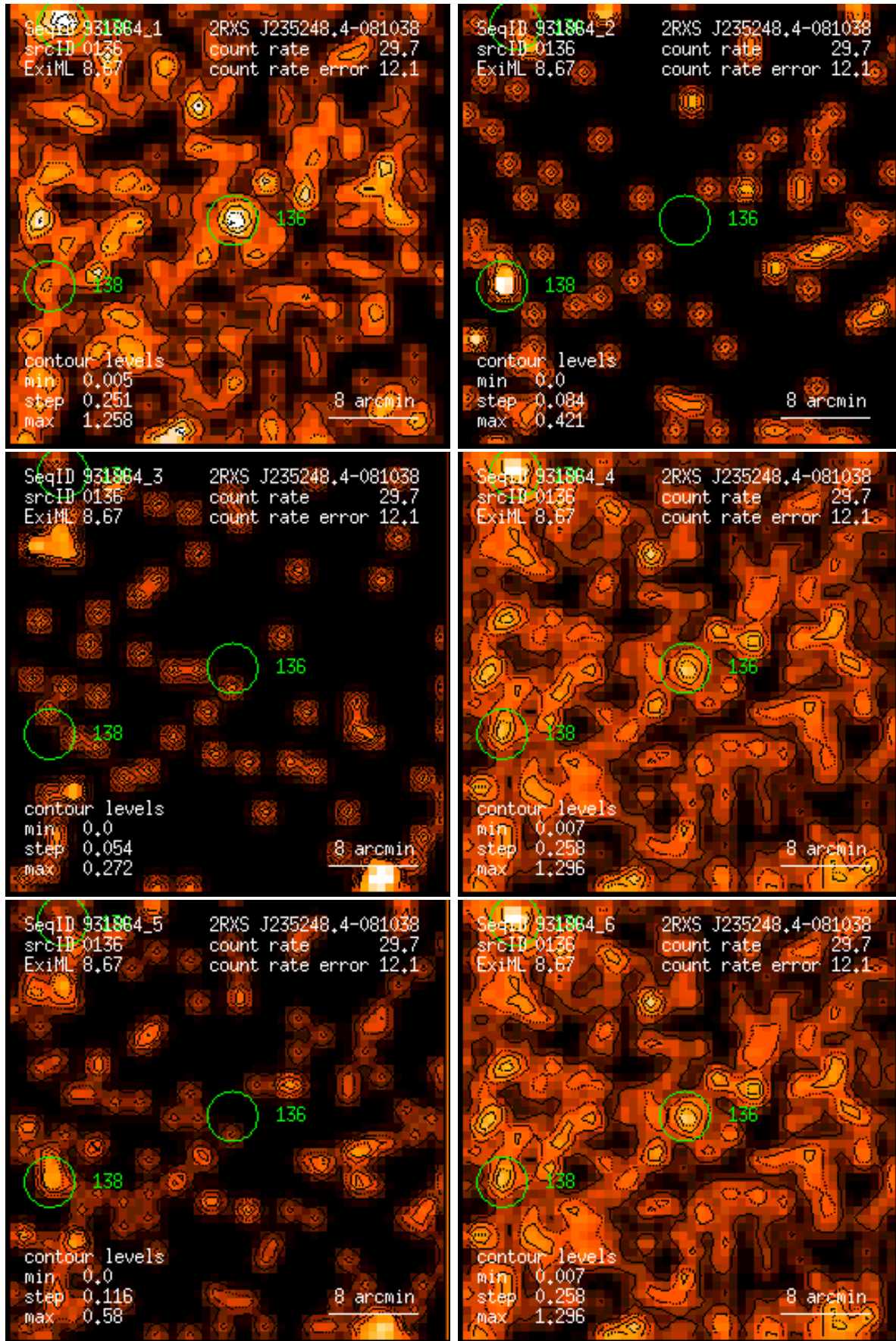
Figure 136: RASS 931864: detection 0136: band rate images, Gaussian filter: (1) PSPC channels 11 – 41, (2) 52 – 90, (3) 91 – 201, (4) 11 – 235, (5) 52 – 201, (6) 11 – 201. Broad band rates in counts/ks. Band rate contour levels in counts/ks/arcmin 2 .
