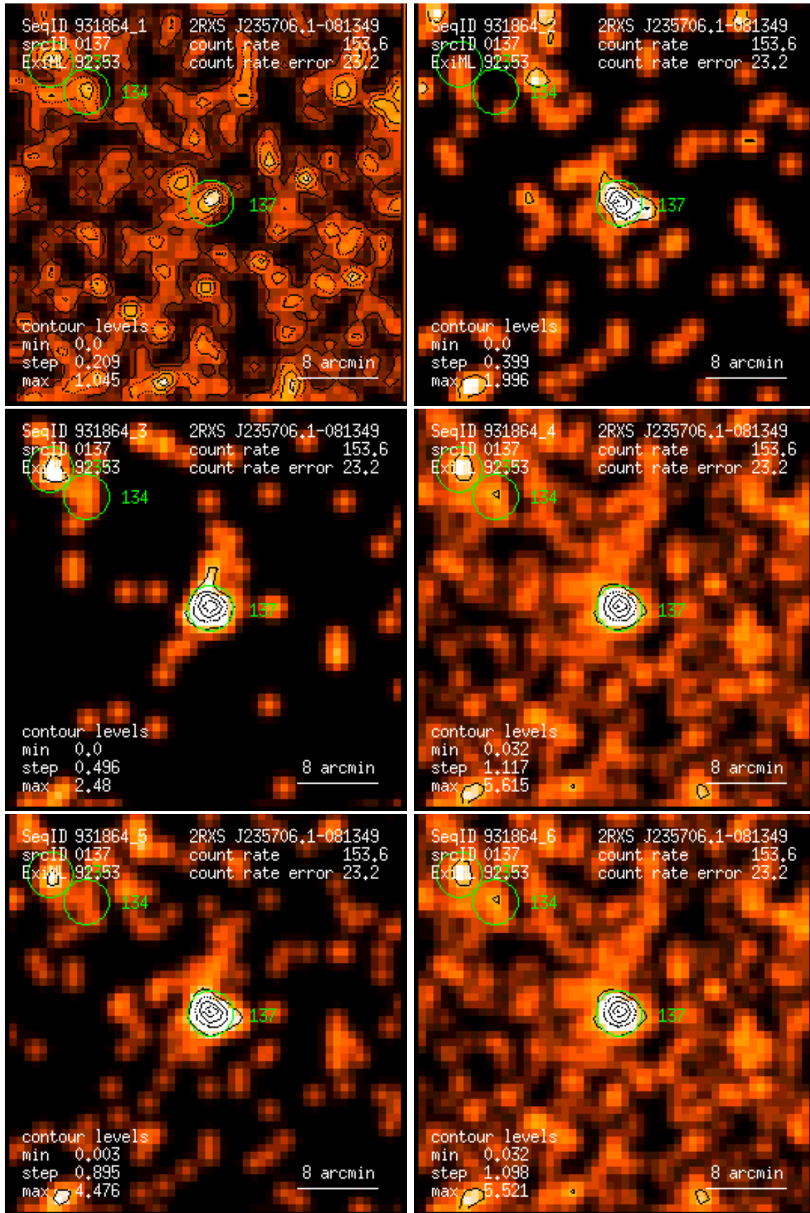
Figure 137: RASS 931864: detection 0137: band rate images, Gaussian filter: (1) PSPC channels 11 – 41, (2) 52 – 90, (3) 91 – 201, (4) 11 – 235, (5) 52 – 201, (6) 11 – 201. Broad band rates in counts/ks. Band rate contour levels in counts/ks/arcmin 2 .
