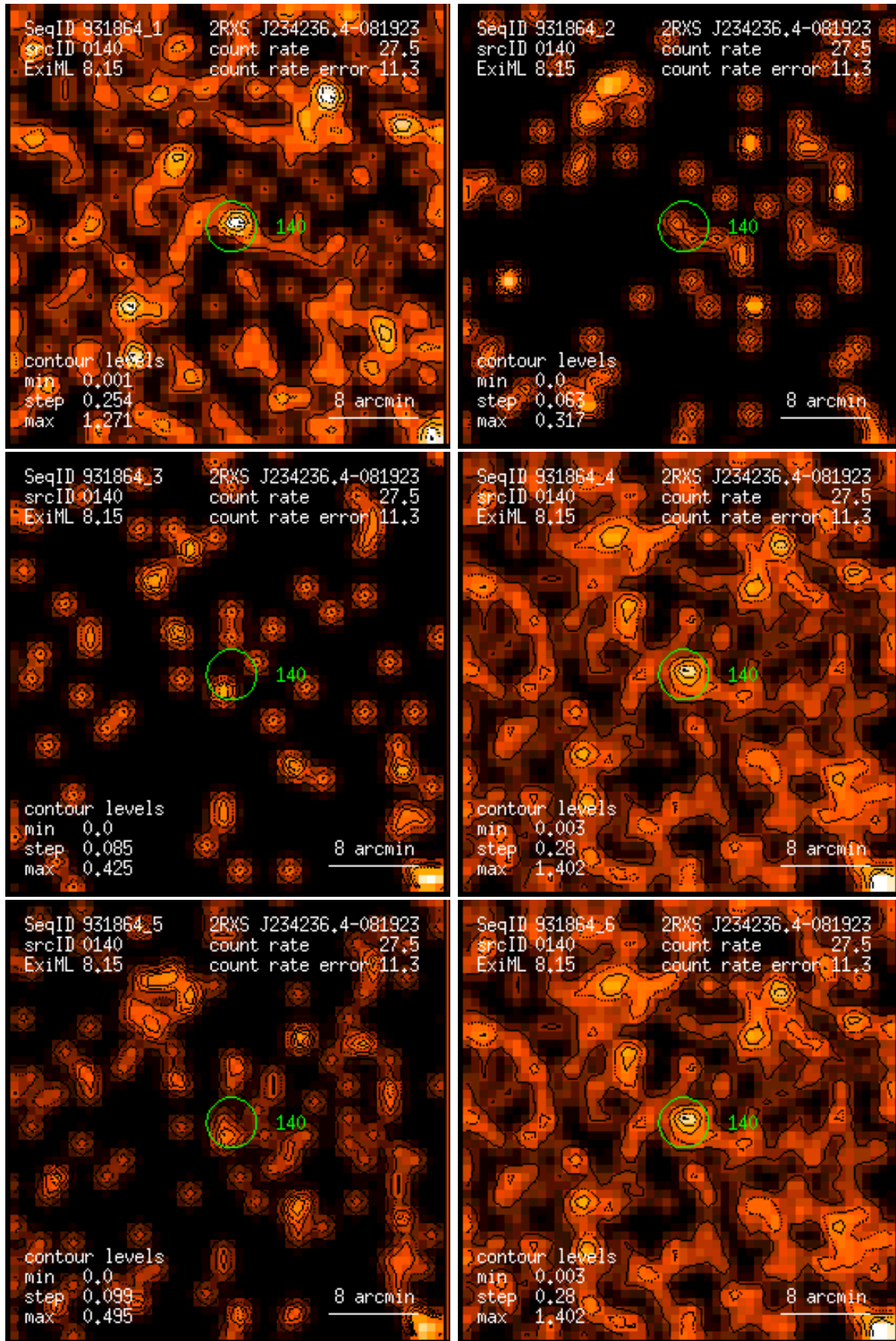
Figure 140: RASS 931864: detection 0140: band rate images, Gaussian filter: (1) PSPC channels 11 – 41, (2) 52 – 90, (3) 91 – 201, (4) 11 – 235, (5) 52 – 201, (6) 11 – 201. Broad band rates in counts/ks. Band rate contour levels in counts/ks/arcmin 2 .
