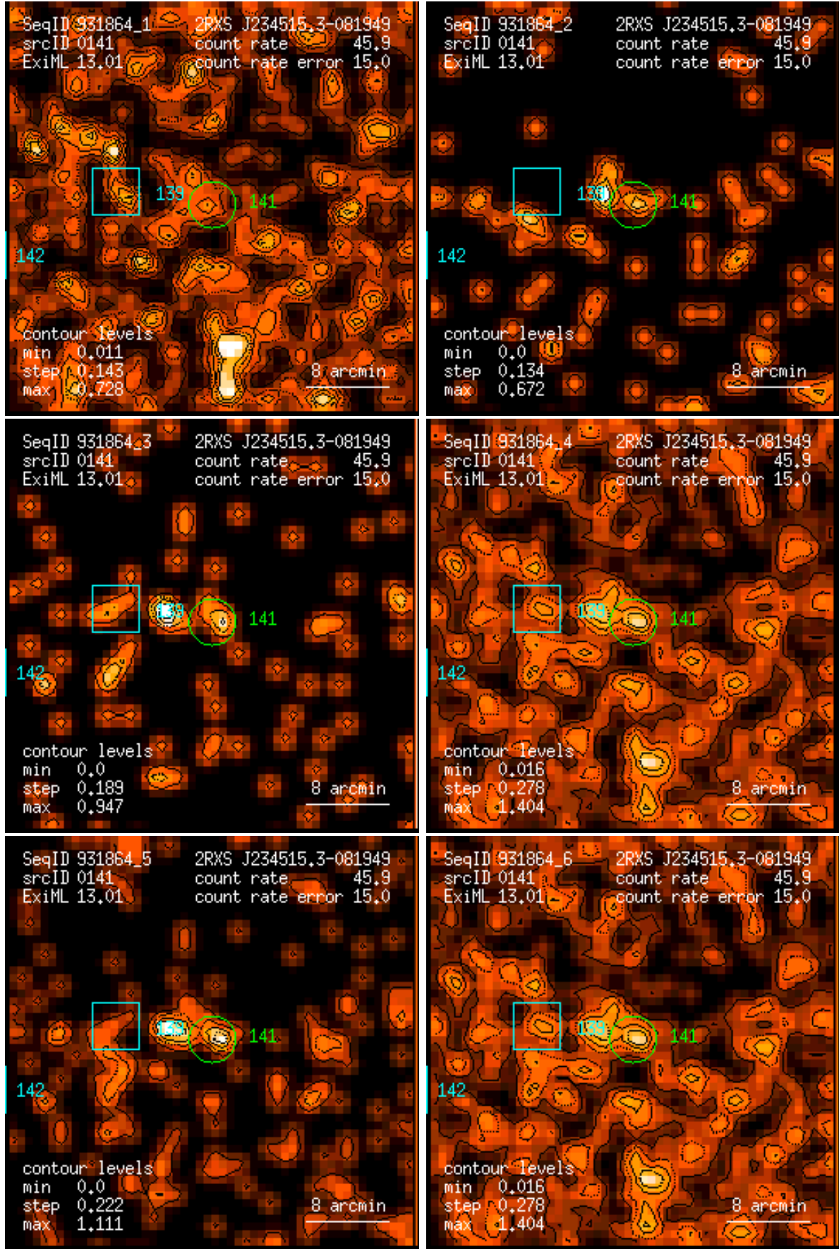
Figure 141: RASS 931864: detection 0141: band rate images, Gaussian filter: (1) PSPC channels 11 – 41, (2) 52 – 90, (3) 91 – 201, (4) 11 – 235, (5) 52 – 201, (6) 11 – 201. Broad band rates in counts/ks. Band rate contour levels in counts/ks/arcmin 2 .
