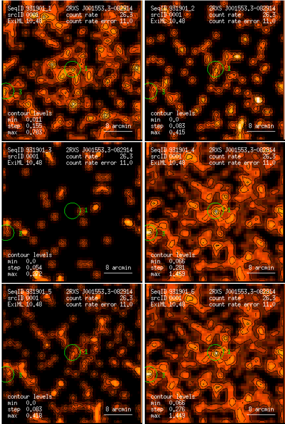
Figure 1: RASS 931901: detection 0001: band rate images, Gaussian filter: (1) PSPC channels 11 – 41, (2) 52 – 90, (3) 91 – 201, (4) 11 – 235, (5) 52 – 201, (6) 11 – 201. Broad band rates in counts/ks. Band rate contour levels in counts/ks/arcmin 2 .
