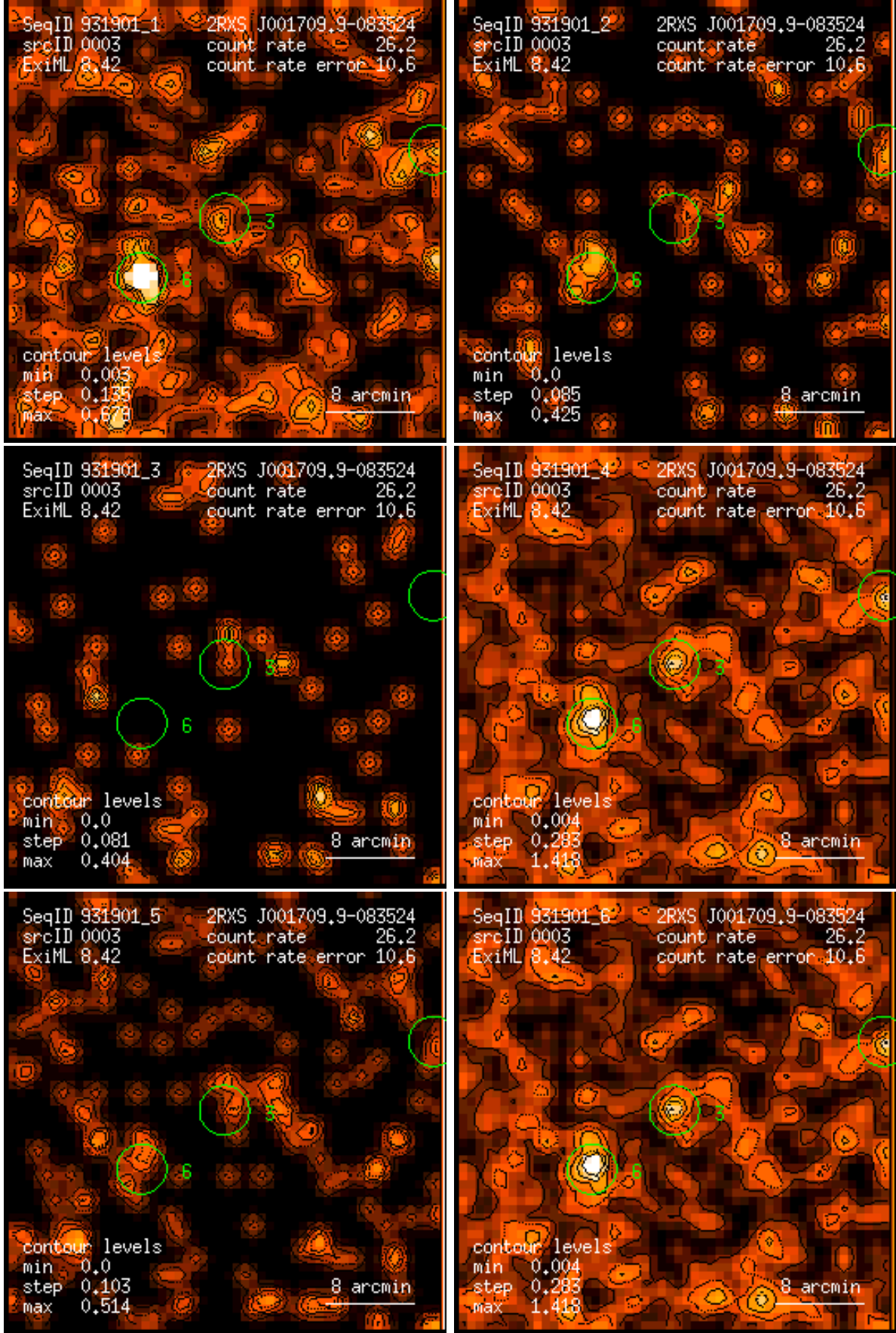
Figure 3: RASS 931901: detection 0003: band rate images, Gaussian filter: (1) PSPC channels 11 – 41, (2) 52 – 90, (3) 91 – 201, (4) 11 – 235, (5) 52 – 201, (6) 11 – 201. Broad band rates in counts/ks. Band rate contour levels in counts/ks/arcmin 2 .
