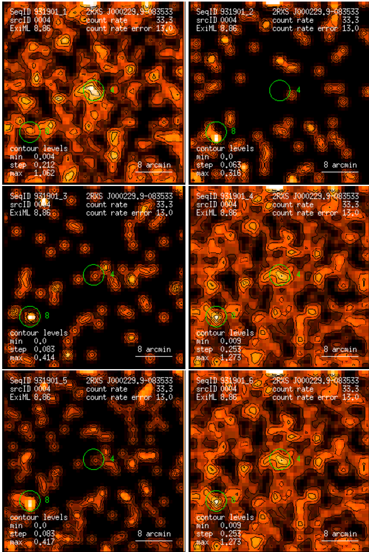
Figure 4: RASS 931901: detection 0004: band rate images, Gaussian filter: (1) PSPC channels 11 – 41, (2) 52 – 90, (3) 91 – 201, (4) 11 – 235, (5) 52 – 201, (6) 11 – 201. Broad band rates in counts/ks. Band rate contour levels in counts/ks/arcmin 2 .
