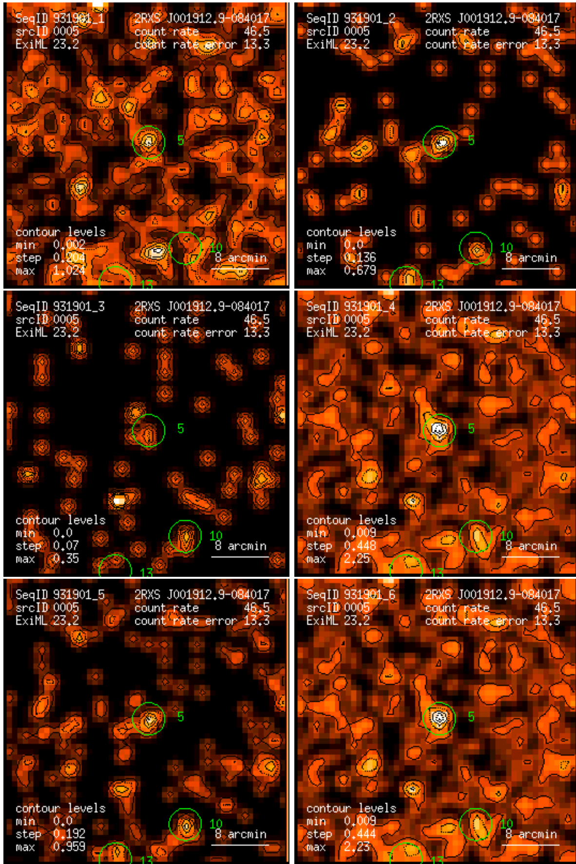
Figure 5: RASS 931901: detection 0005: band rate images, Gaussian filter: (1) PSPC channels 11 – 41, (2) 52 – 90, (3) 91 – 201, (4) 11 – 235, (5) 52 – 201, (6) 11 – 201. Broad band rates in counts/ks. Band rate contour levels in counts/ks/arcmin 2 .
