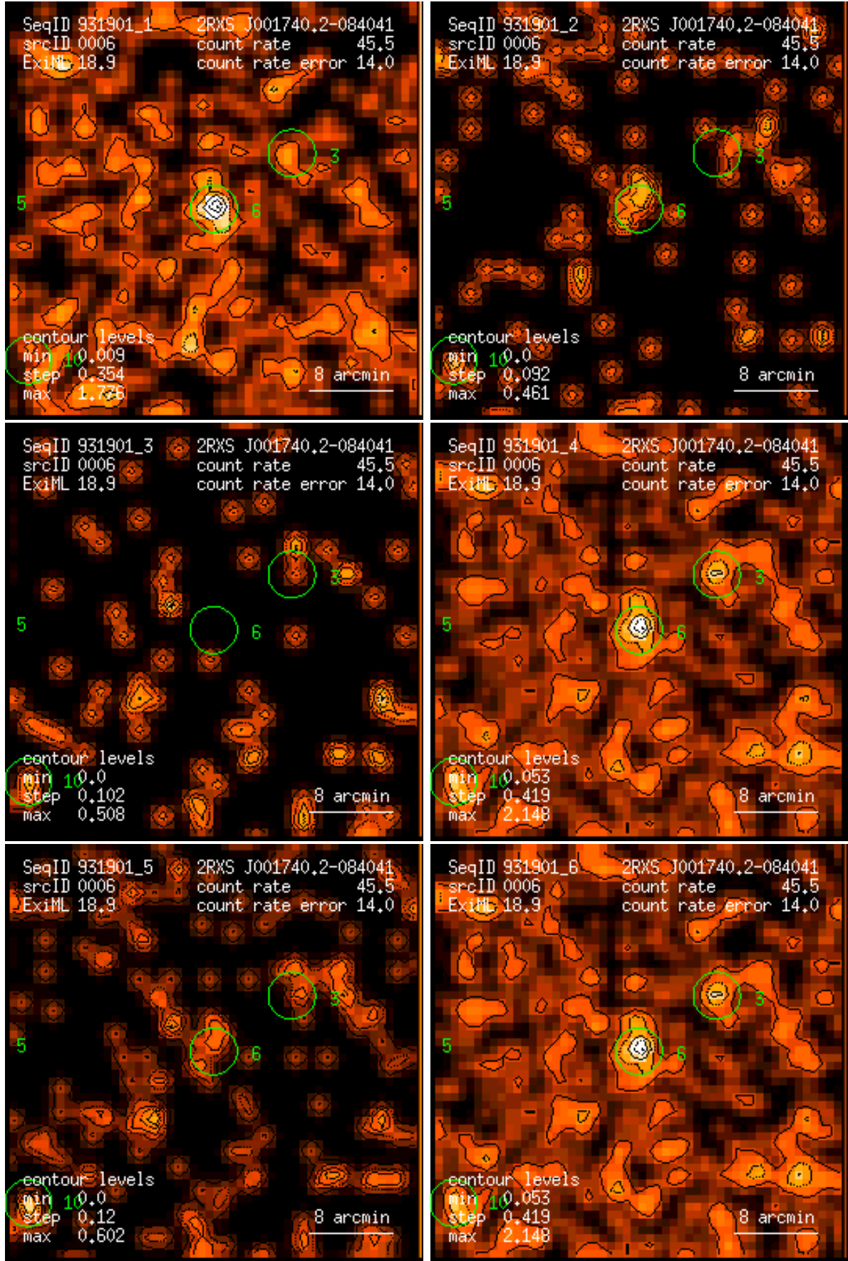
Figure 6: RASS 931901: detection 0006: band rate images, Gaussian filter: (1) PSPC channels 11 – 41, (2) 52 – 90, (3) 91 – 201, (4) 11 – 235, (5) 52 – 201, (6) 11 – 201. Broad band rates in counts/ks. Band rate contour levels in counts/ks/arcmin 2 .
