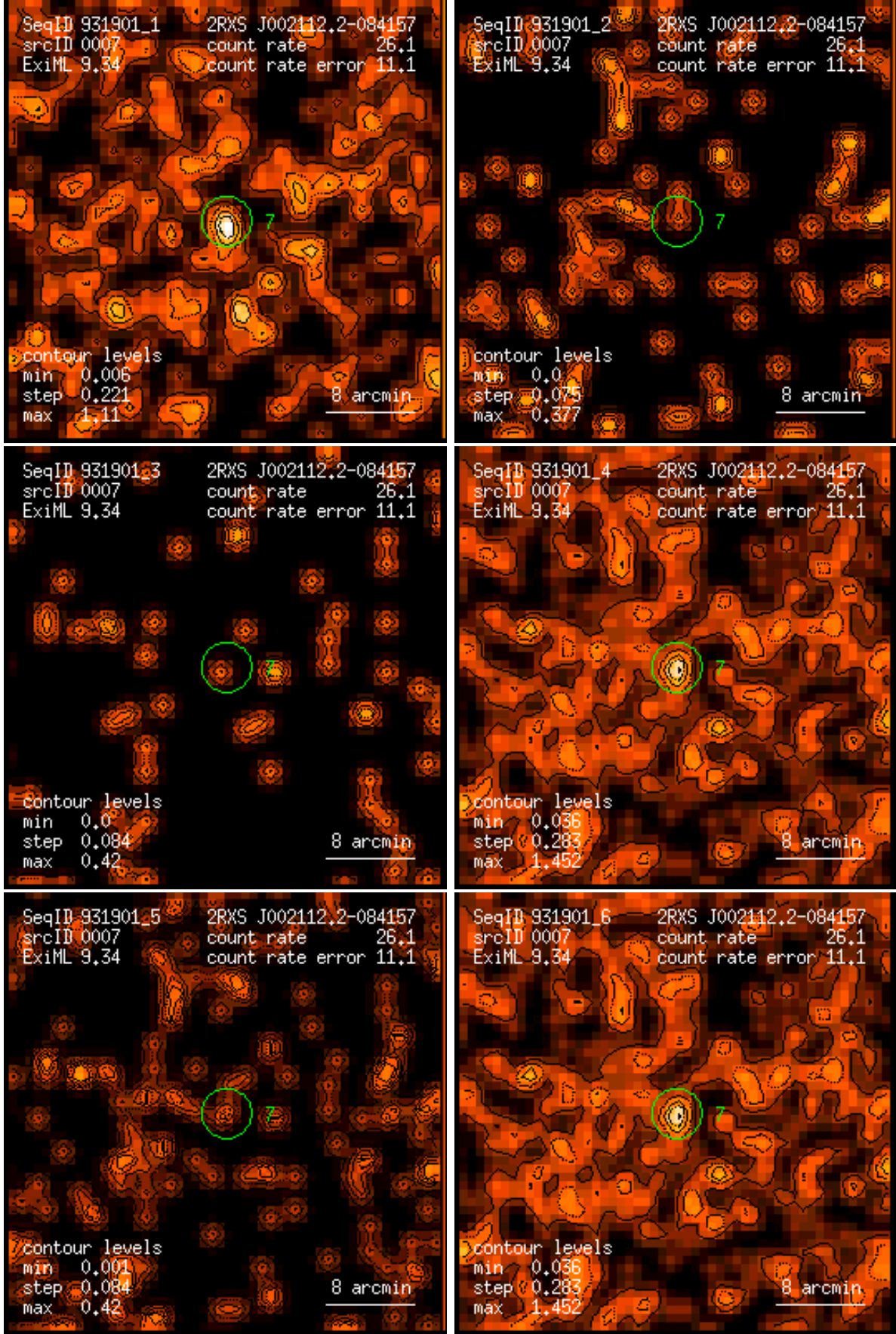
Figure 7: RASS 931901: detection 0007: band rate images, Gaussian filter: (1) PSPC channels 11 – 41, (2) 52 – 90, (3) 91 – 201, (4) 11 – 235, (5) 52 – 201, (6) 11 – 201. Broad band rates in counts/ks. Band rate contour levels in counts/ks/arcmin 2 .
