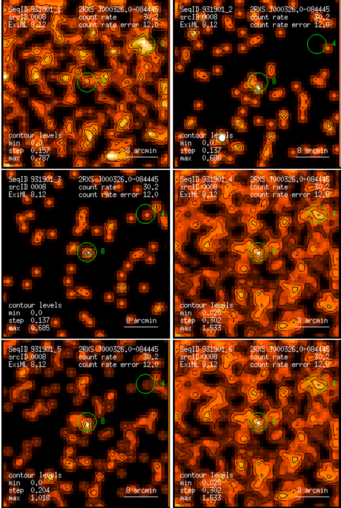
Figure 8: RASS 931901: detection 0008: band rate images, Gaussian filter: (1) PSPC channels 11 – 41, (2) 52 – 90, (3) 91 – 201, (4) 11 – 235, (5) 52 – 201, (6) 11 – 201. Broad band rates in counts/ks. Band rate contour levels in counts/ks/arcmin 2 .
