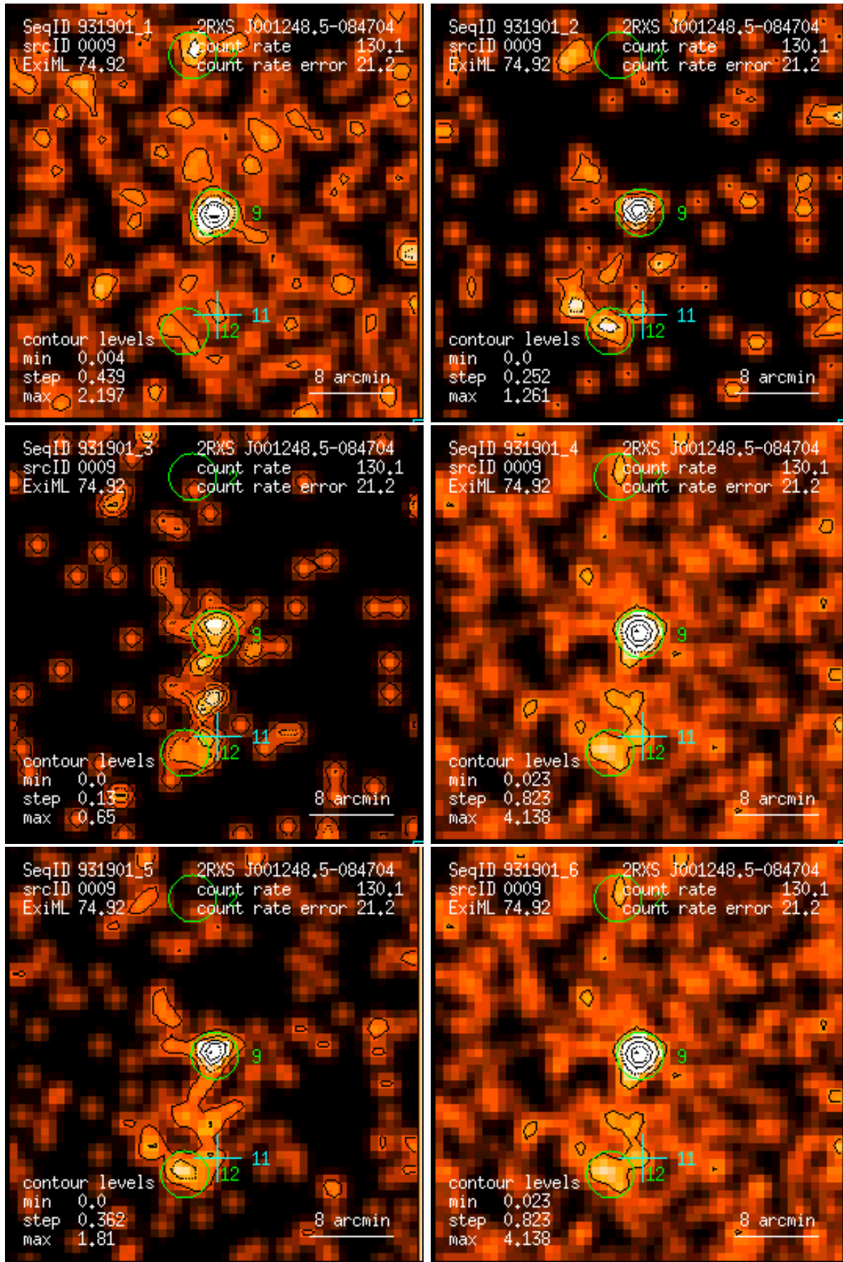
Figure 9: RASS 931901: detection 0009: band rate images, Gaussian filter: (1) PSPC channels 11 – 41, (2) 52 – 90, (3) 91 – 201, (4) 11 – 235, (5) 52 – 201, (6) 11 – 201. Broad band rates in counts/ks. Band rate contour levels in counts/ks/arcmin 2 .
