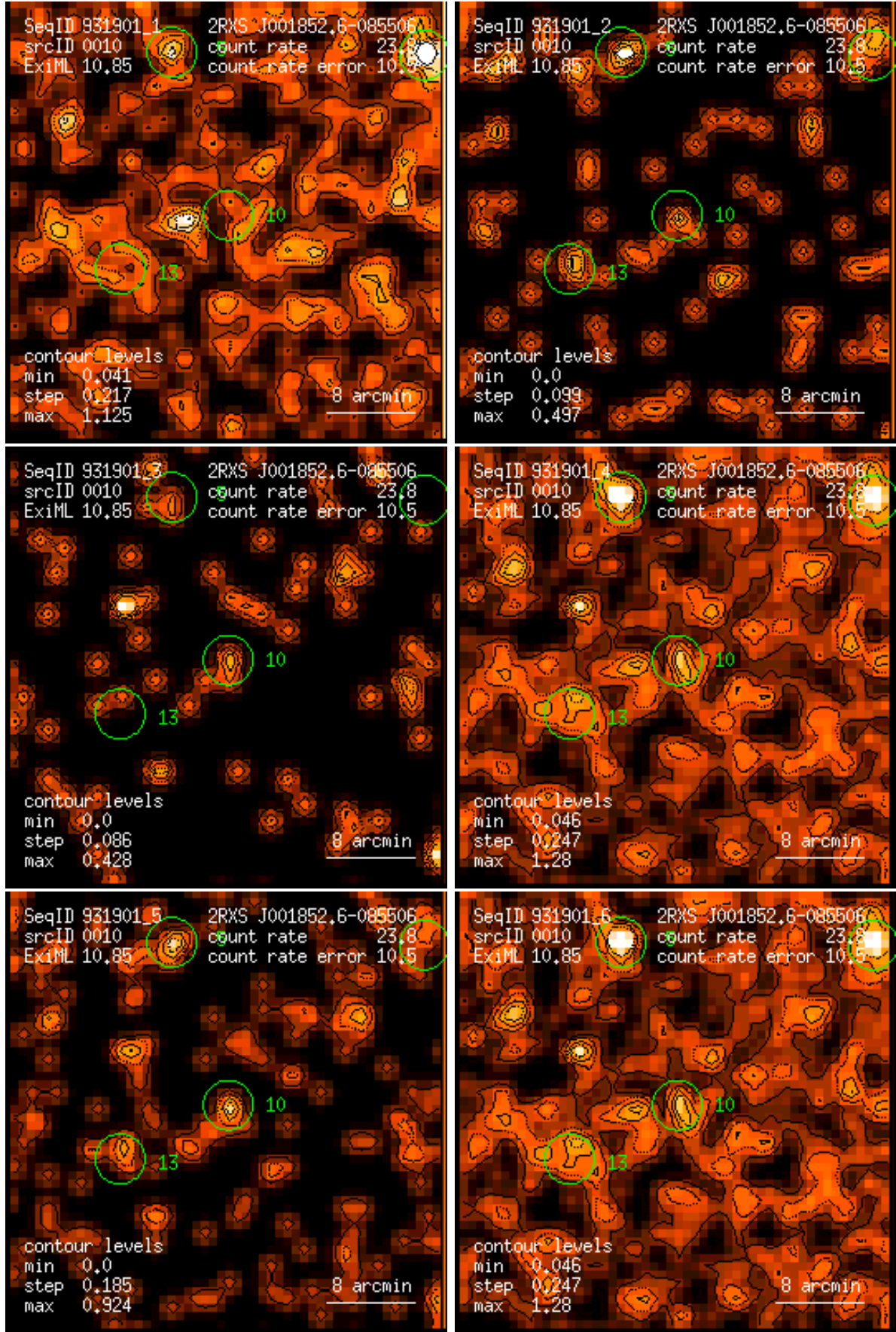
Figure 10: RASS 931901: detection 0010: band rate images, Gaussian filter: (1) PSPC channels 11 – 41, (2) 52 – 90, (3) 91 – 201, (4) 11 – 235, (5) 52 – 201, (6) 11 – 201. Broad band rates in counts/ks. Band rate contour levels in counts/ks/arcmin 2 .
